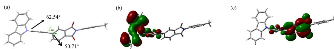
Figure 1. (a) Single-crystal structure of PI-Cz; (b) HOMO distribution calculated on the crystallographic geometry; (c) LUMO distribution calculated on the crystallographic geometry.
