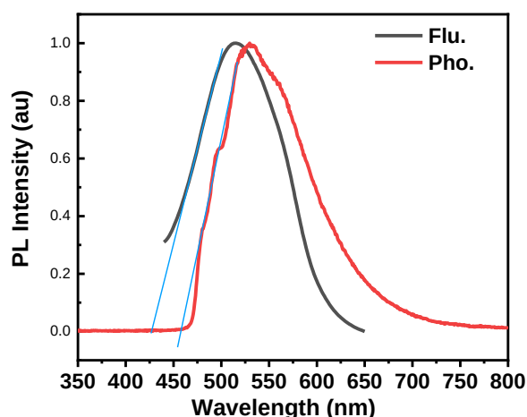
Figure 3. Fluorescence and phosphorescence spectra of PI-Cz in THF.
