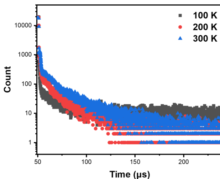
Figure 7. Photoluminescence lifetime of PI-Cz films at different temperatures.
