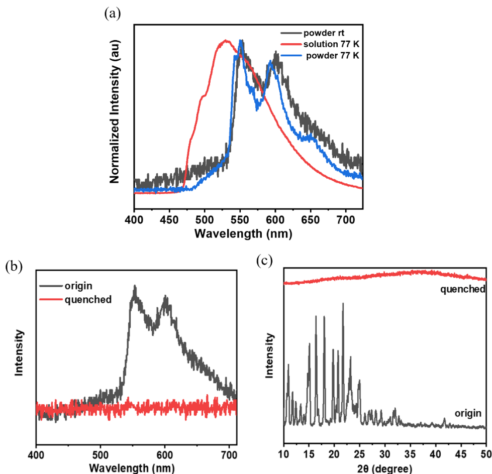
Figure 5. (a) Phosphorescence spectra of PI-Cz in the powder state at room temperature and at 77 K, and in dilute solution at 77 K; (b) phosphorescence spectra of PI-Cz powder before and after melt quenching; (c) powder X-ray diffraction (PXRD) patterns of the powder and the melt-quenched solid.
