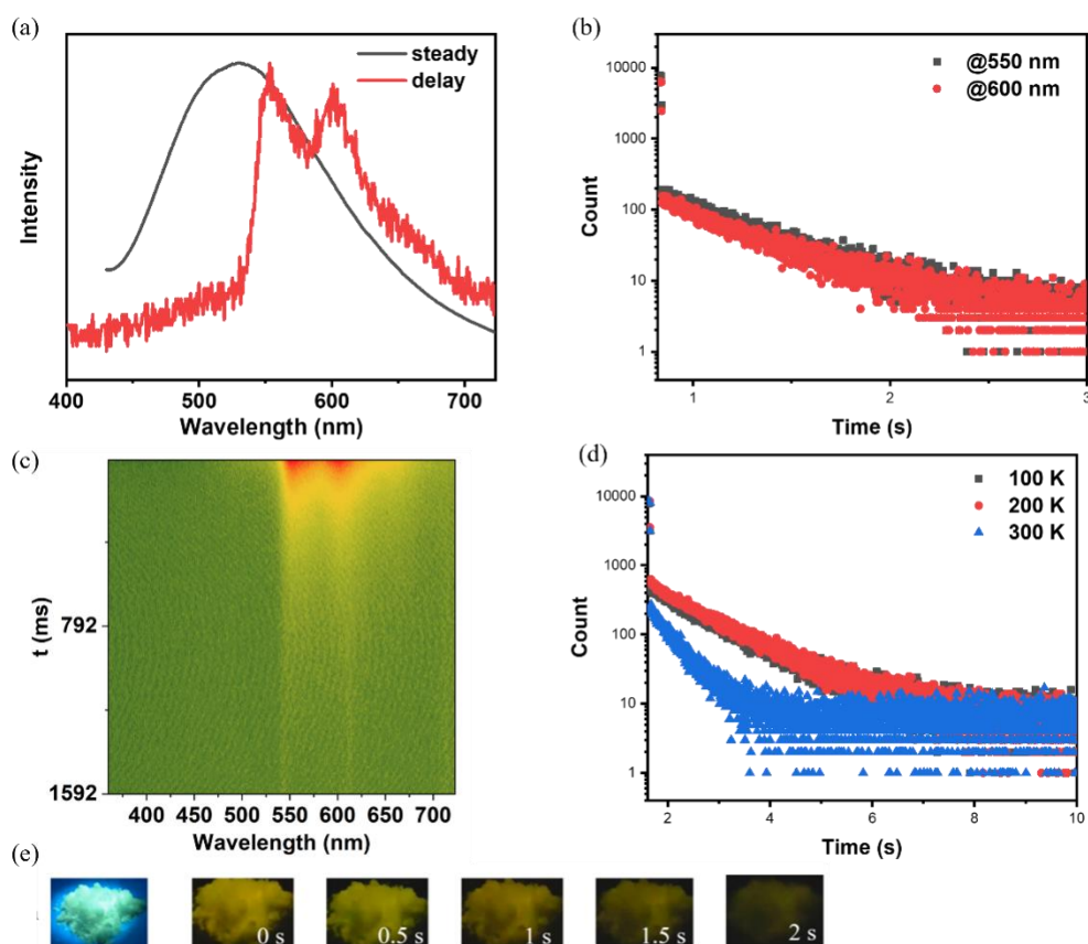
Figure 4. (a) Steady-state and delayed emission spectra of PI-Cz; (b) room-temperature emission lifetimes monitored at 550 nm and 600 nm; (c) time-resolved emission spectra; (d) temperature-dependent lifetime at 550 nm; (e) photographs of PI-Cz under UV irradiation and after removal of the UV source.
