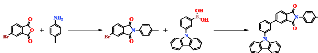
Scheme 1. Synthetic pathway to PI-Cz via imide formation and Suzuki–Miyaura cross-coupling.
