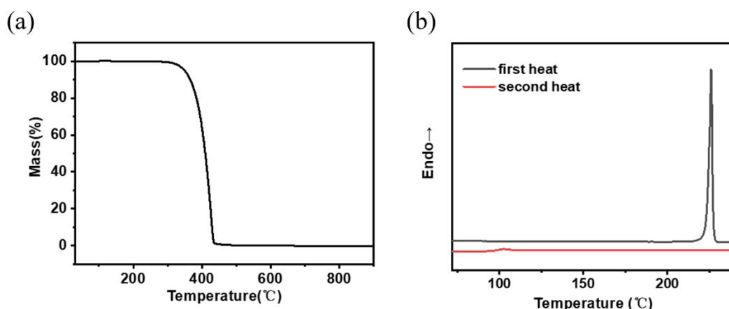
Figure8. (a) T_g curve of PI-Cz; (b) DSC curve of PI-Cz.
