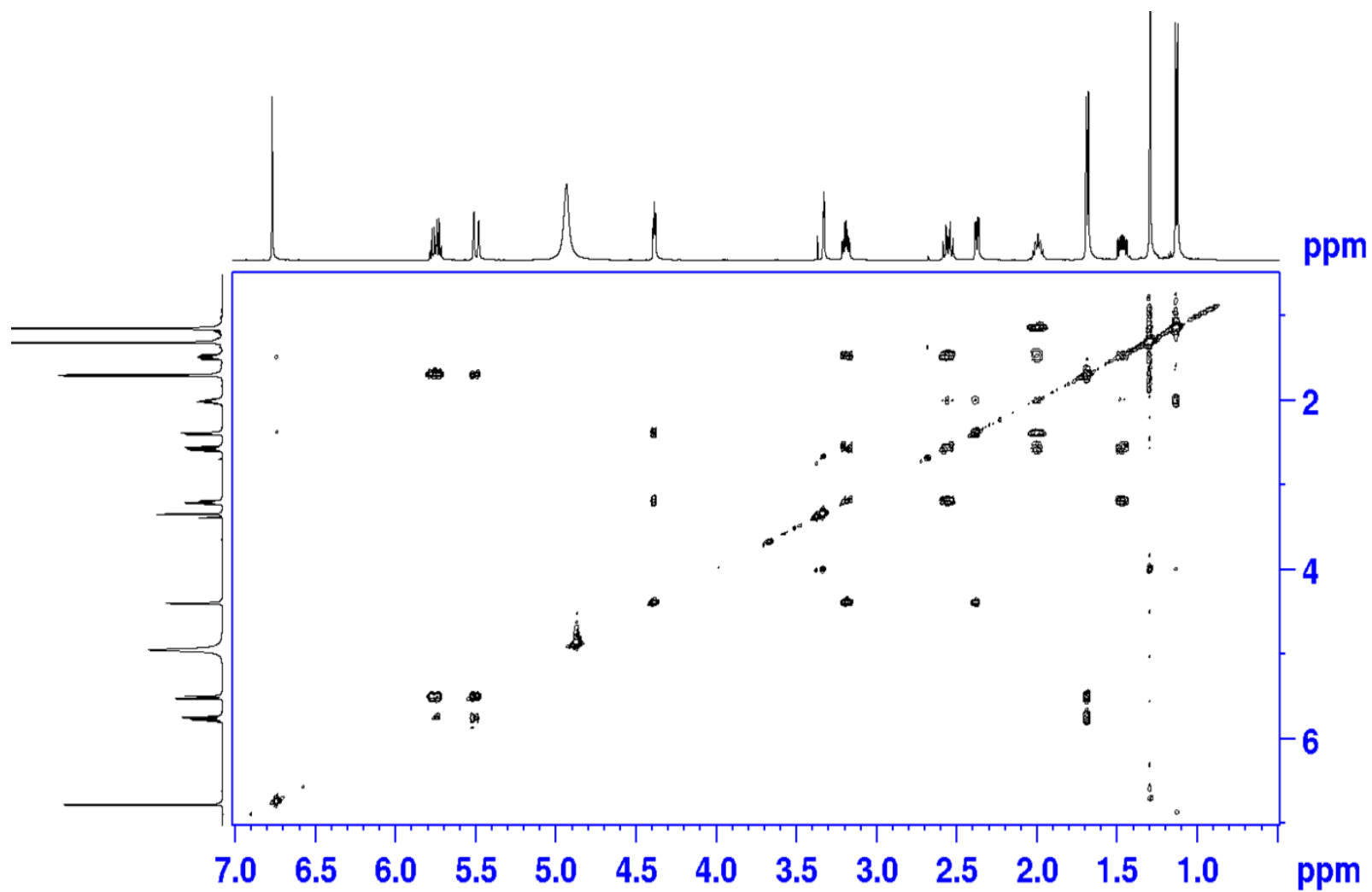
Figure S3. ^1\text{H} - ^1\text{H} COSY spectrum of 1 (500 MHz, \text{CD}_3\text{OD} )
