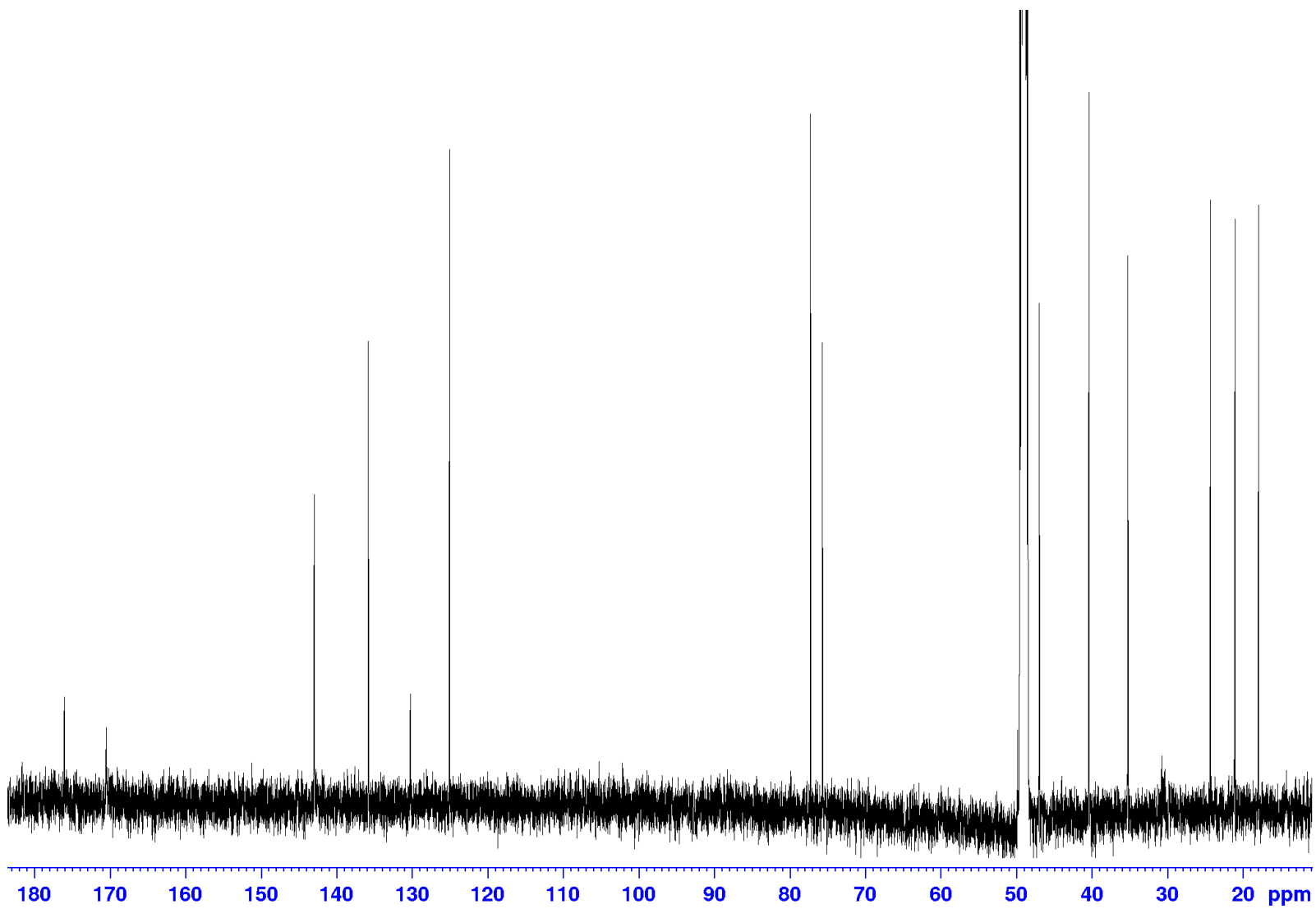
Figure S2. ^{13}\text{C} NMR spectrum of 1 (125 MHz, \text{CD}_3\text{OD} )
