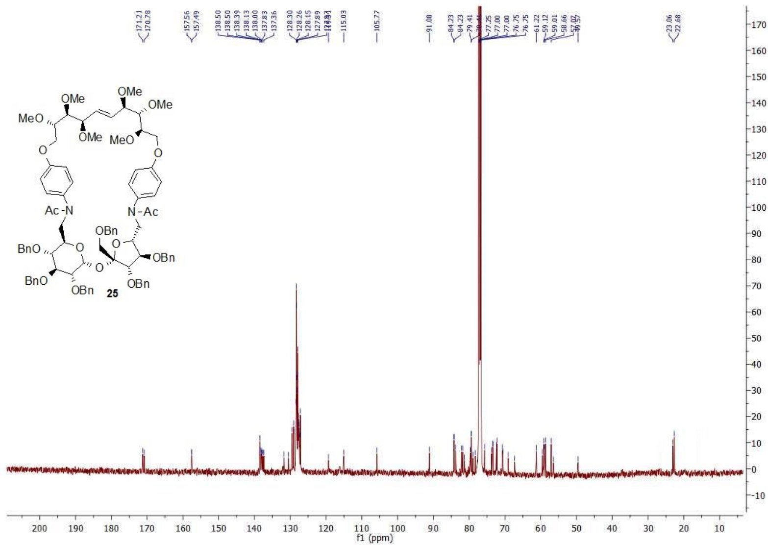
Figure S28 13 C NMR spectrum of compound 25 .
