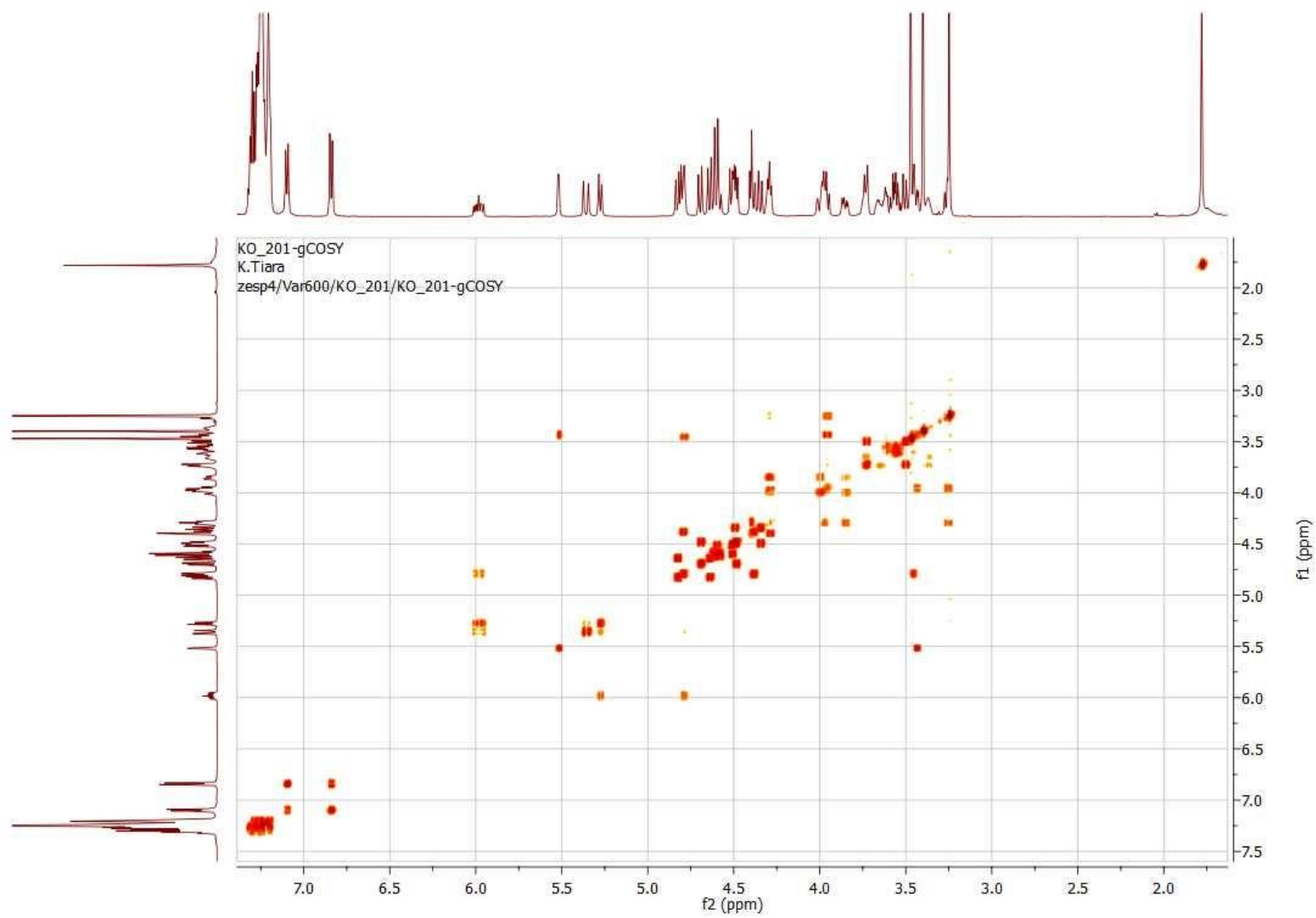
Figure S19 gCOSY spectrum of compound 22 .
