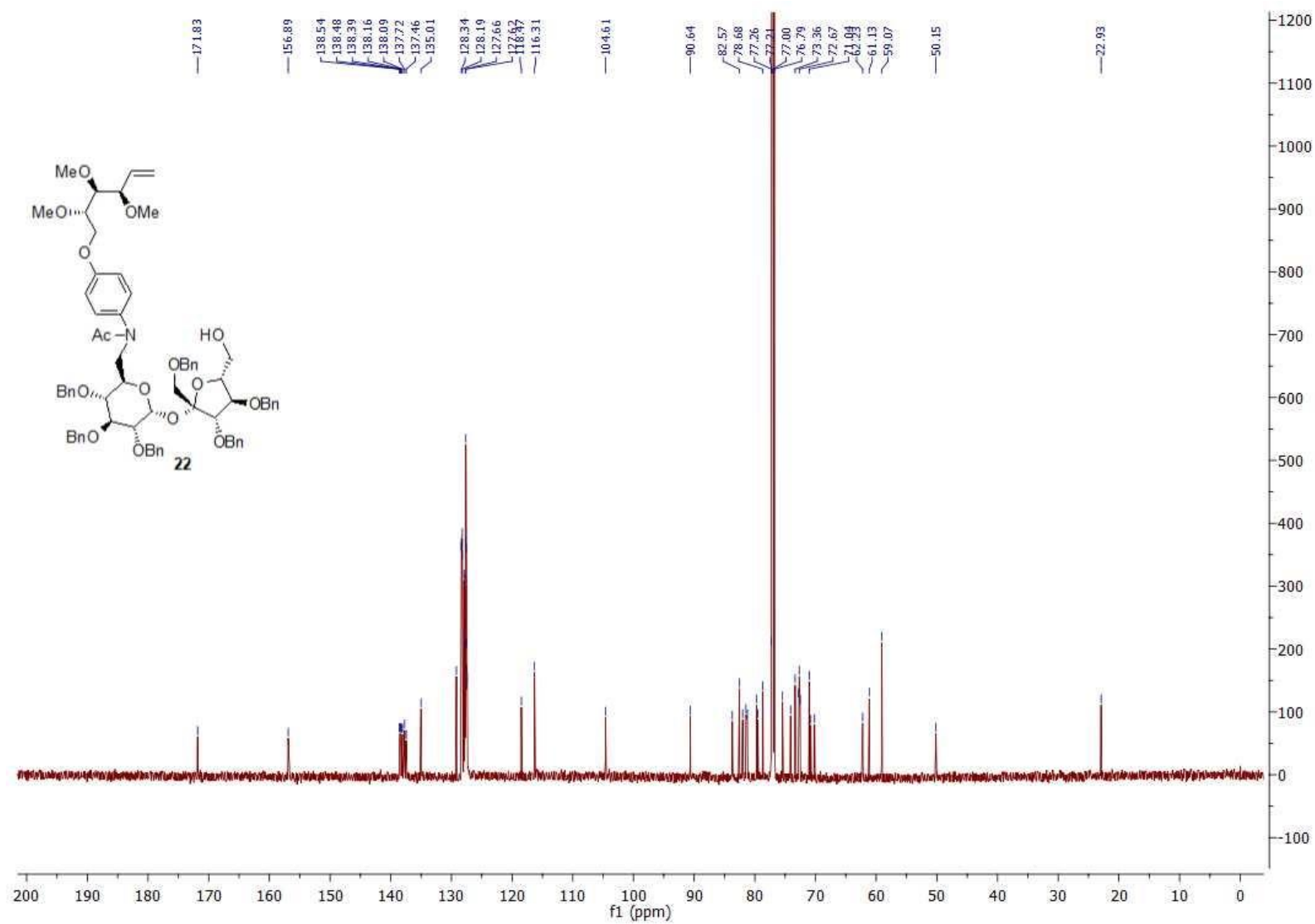
Figure S18 ^{13}\text{C} NMR spectrum of compound 22.
