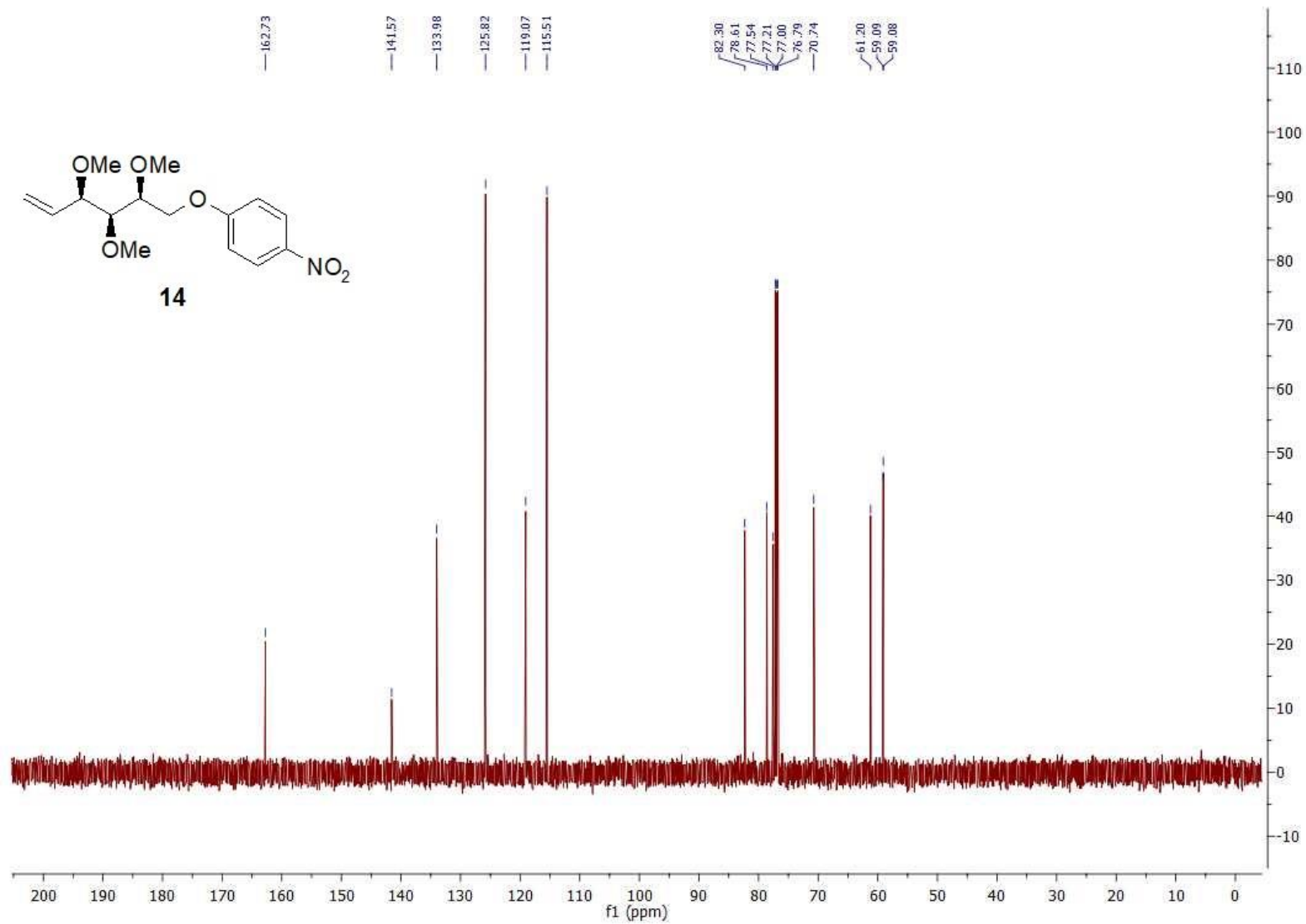
Figure S2 13 C NMR spectrum of compound 14 .
