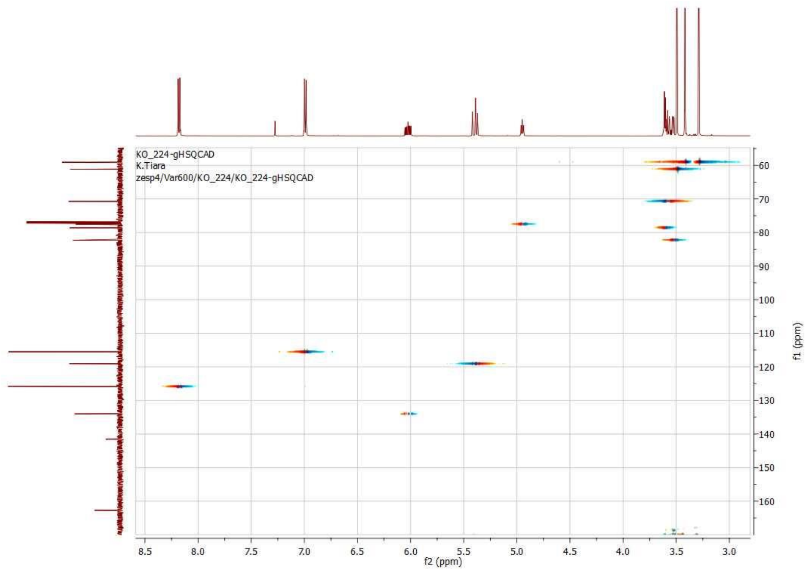
Figure S4 gHSQCAD spectrum of compound 14 .
