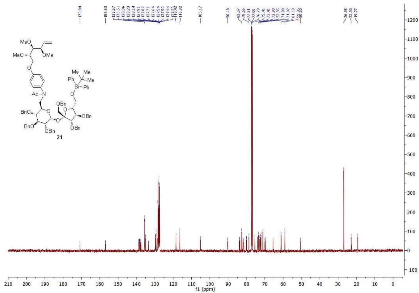
Figure S12 ^{13}\text{C} NMR spectrum of compound 21 .
