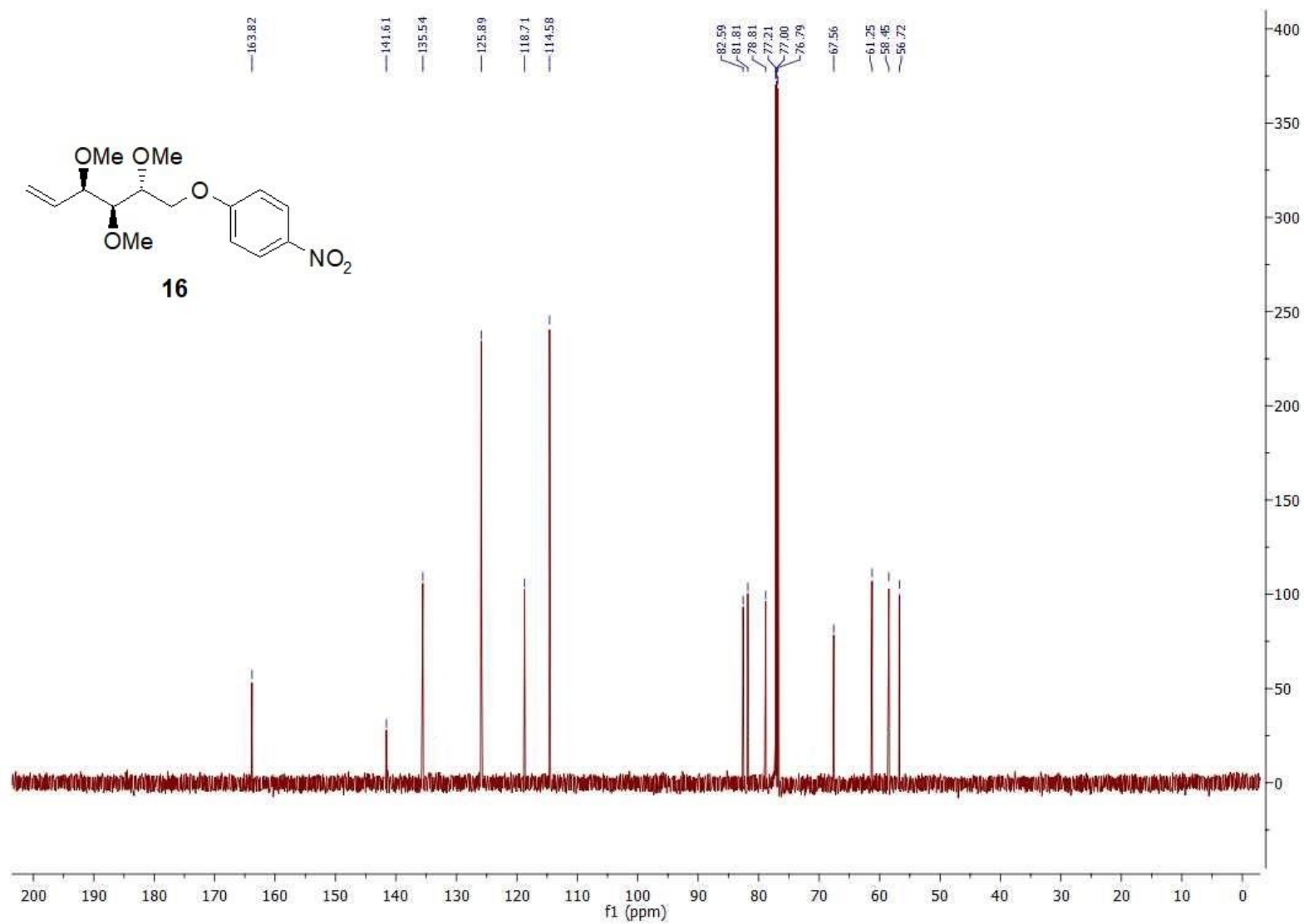
Figure S7 13 C NMR spectrum of compound 16 .
