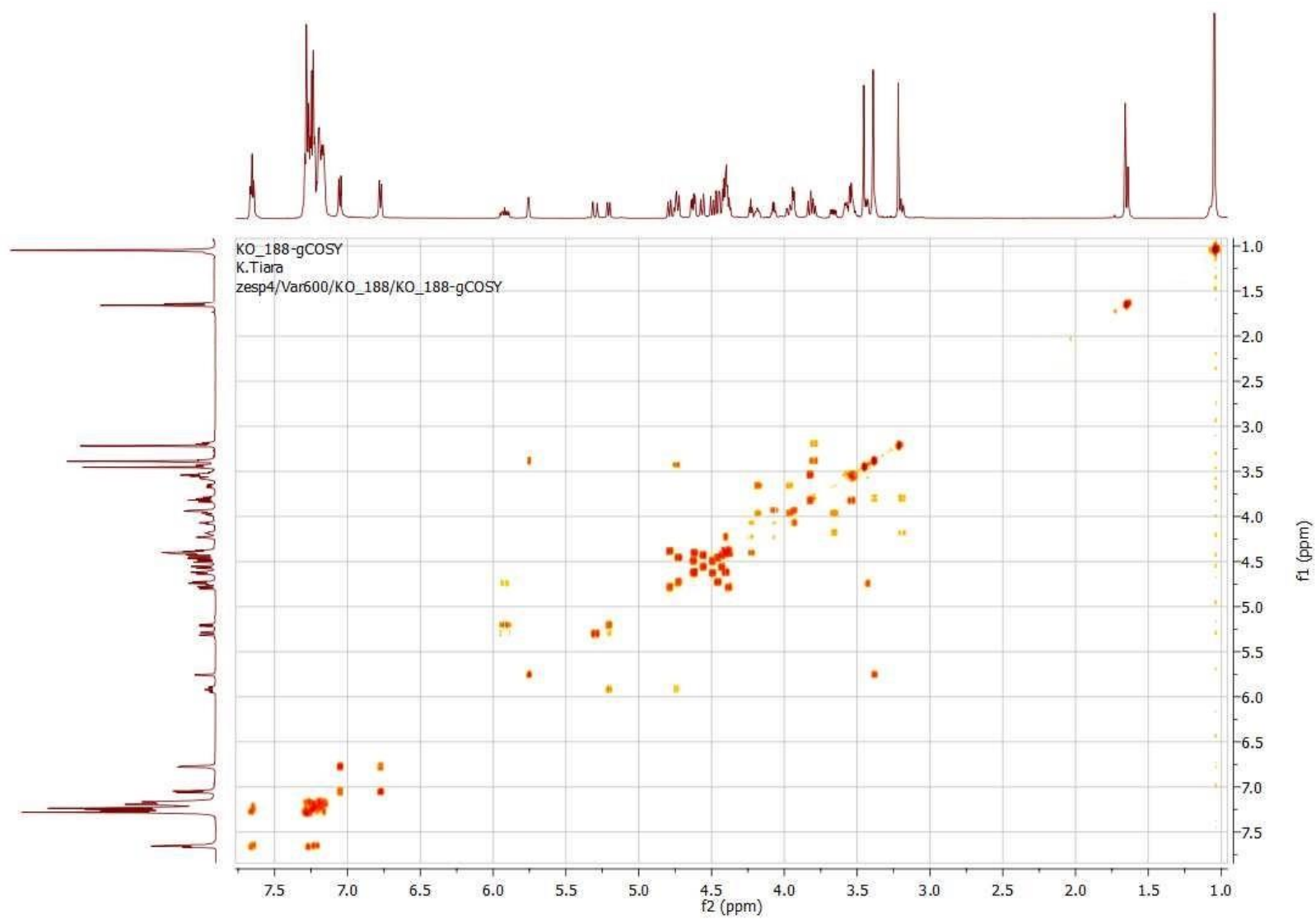
Figure S13 COSY spectrum of compound 21 .
