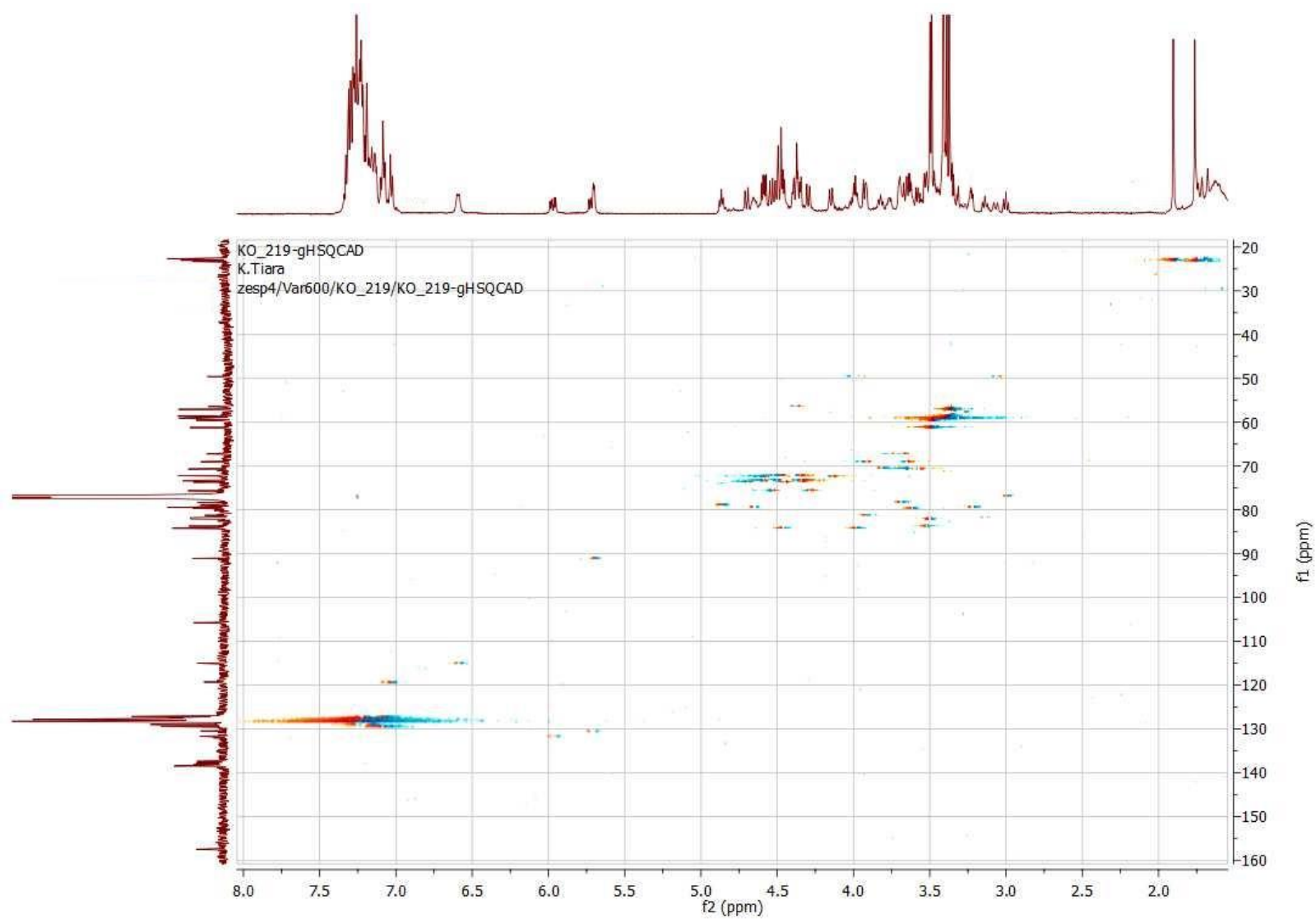
Figure S30 gHSQCAD spectrum of compound 25 .
