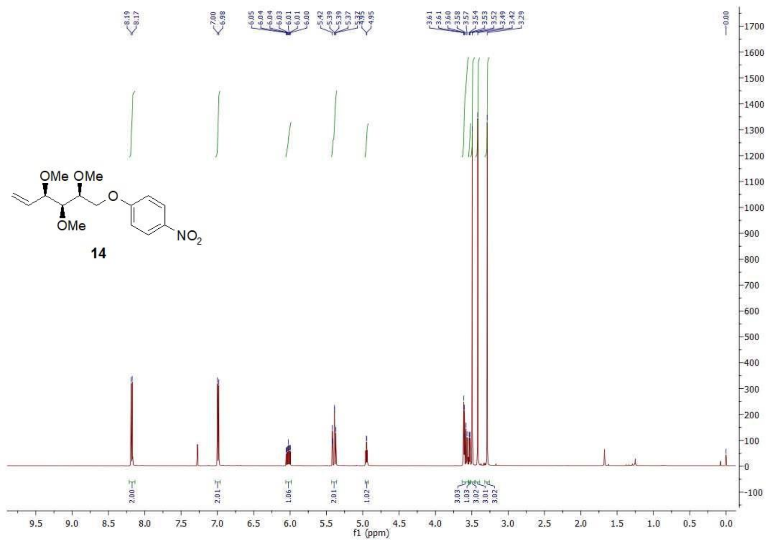
Figure S1 ^1\text{H} NMR spectrum of compound 14 .
