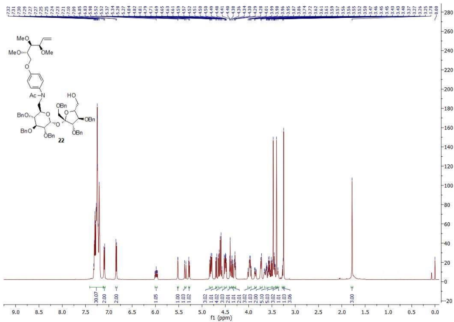
Figure S16 1 H NMR spectrum of compound 22.
