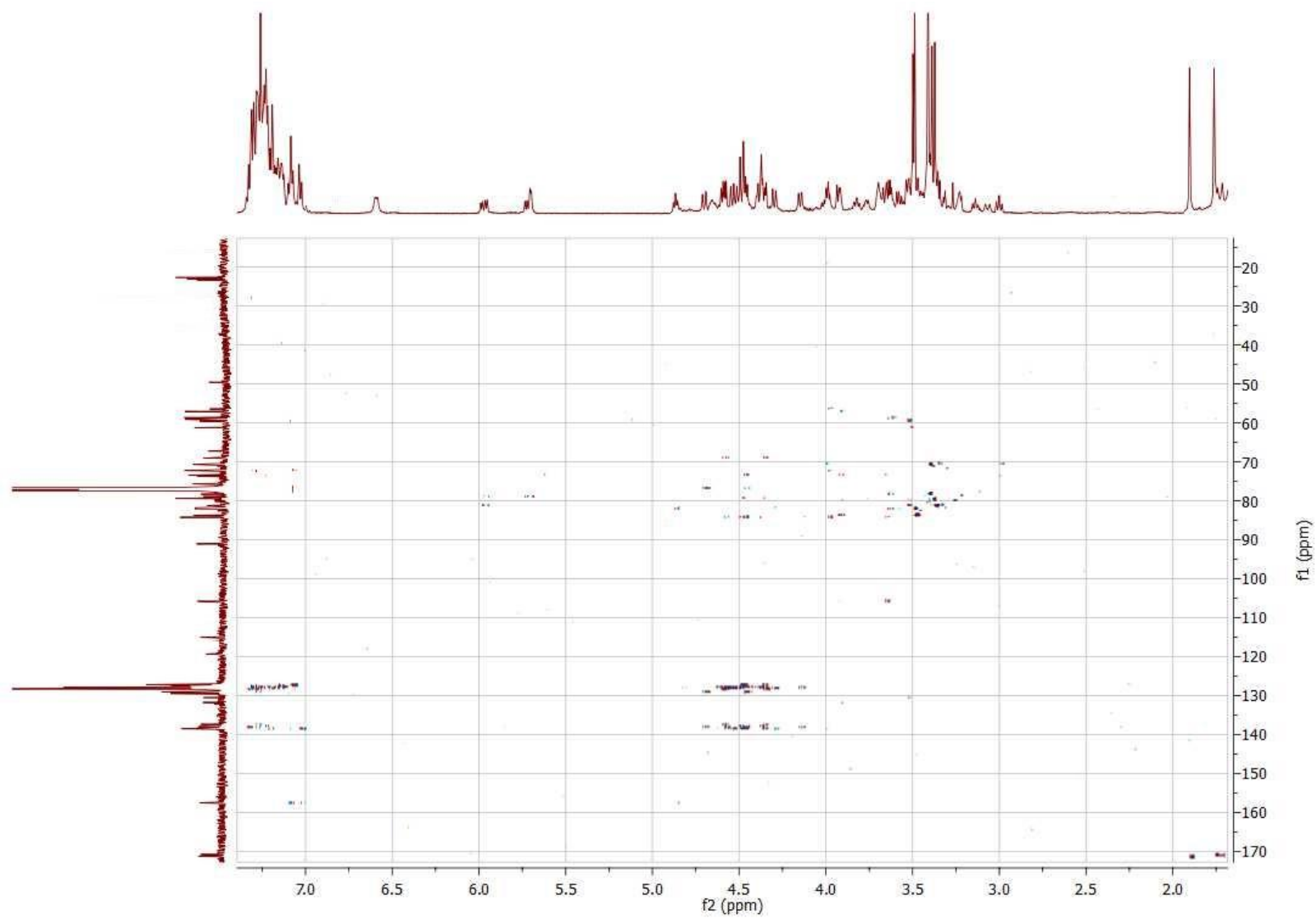
Figure S31 gHMBCAD NMR spectrum of compound 25 .
