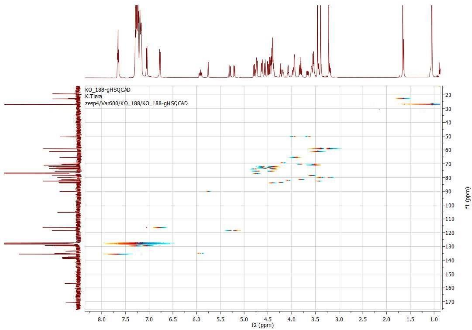
Figure S14 gHSQCAD spectrum of compound 21 .
