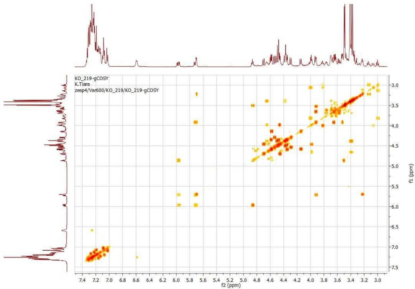
Figure S29 gCOSY spectrum of compound 25 .
