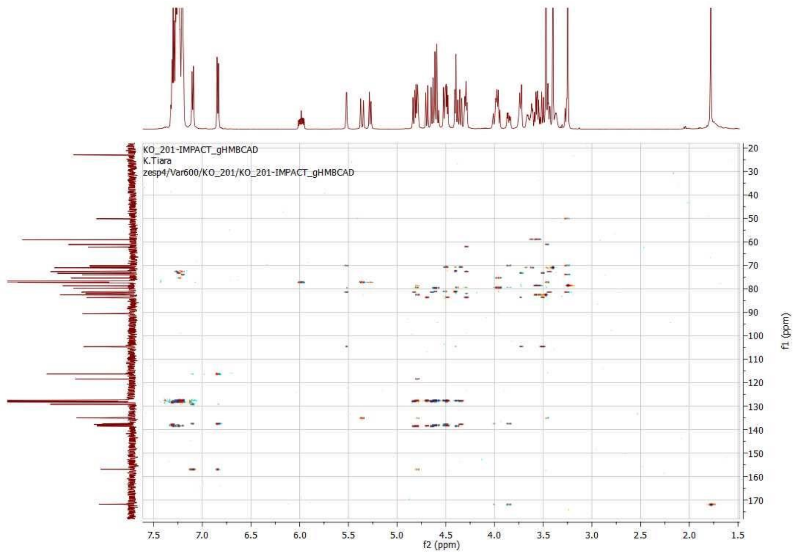
Figure S21 gHMBCAD spectrum of compound 22 .
