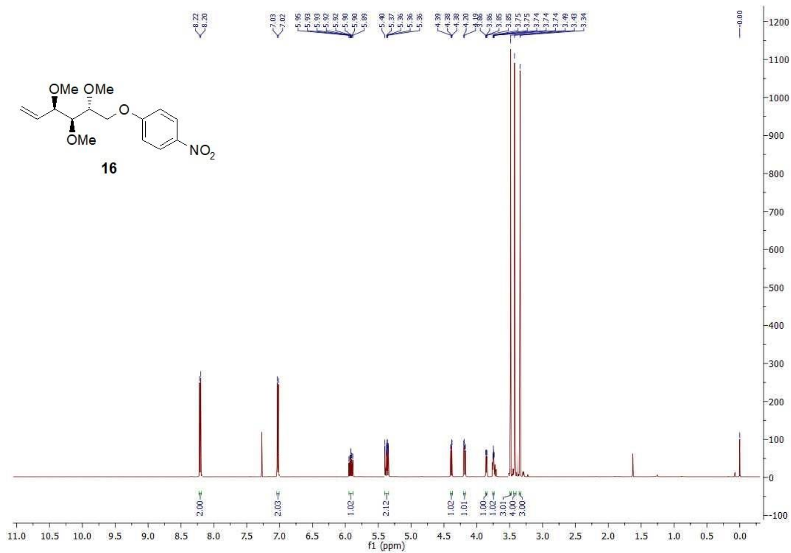
Figure S6 1 H NMR spectrum of compound 16 .
