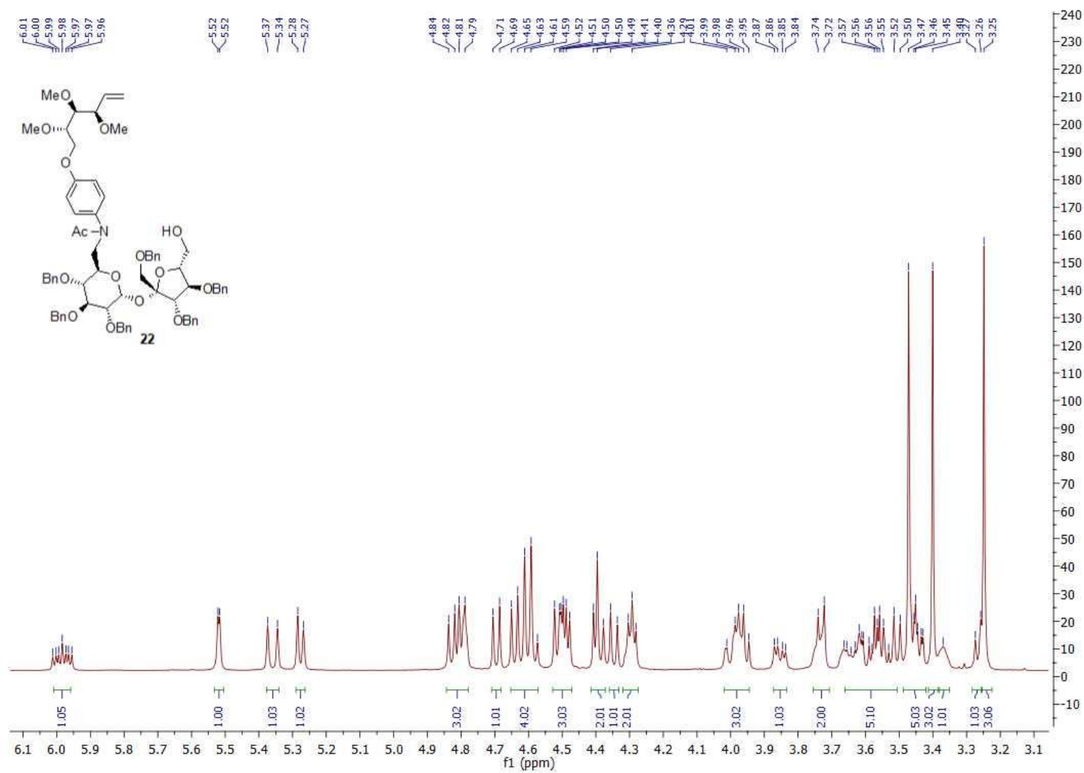
Figure S17 ^1\text{H} NMR spectrum (aliphatic part) of compound 22 .
