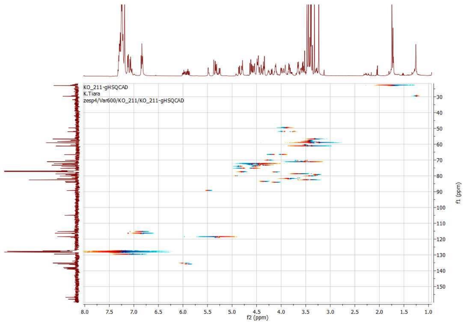
Figure S25 gHSQCAD NMR spectrum of compound 24 .
