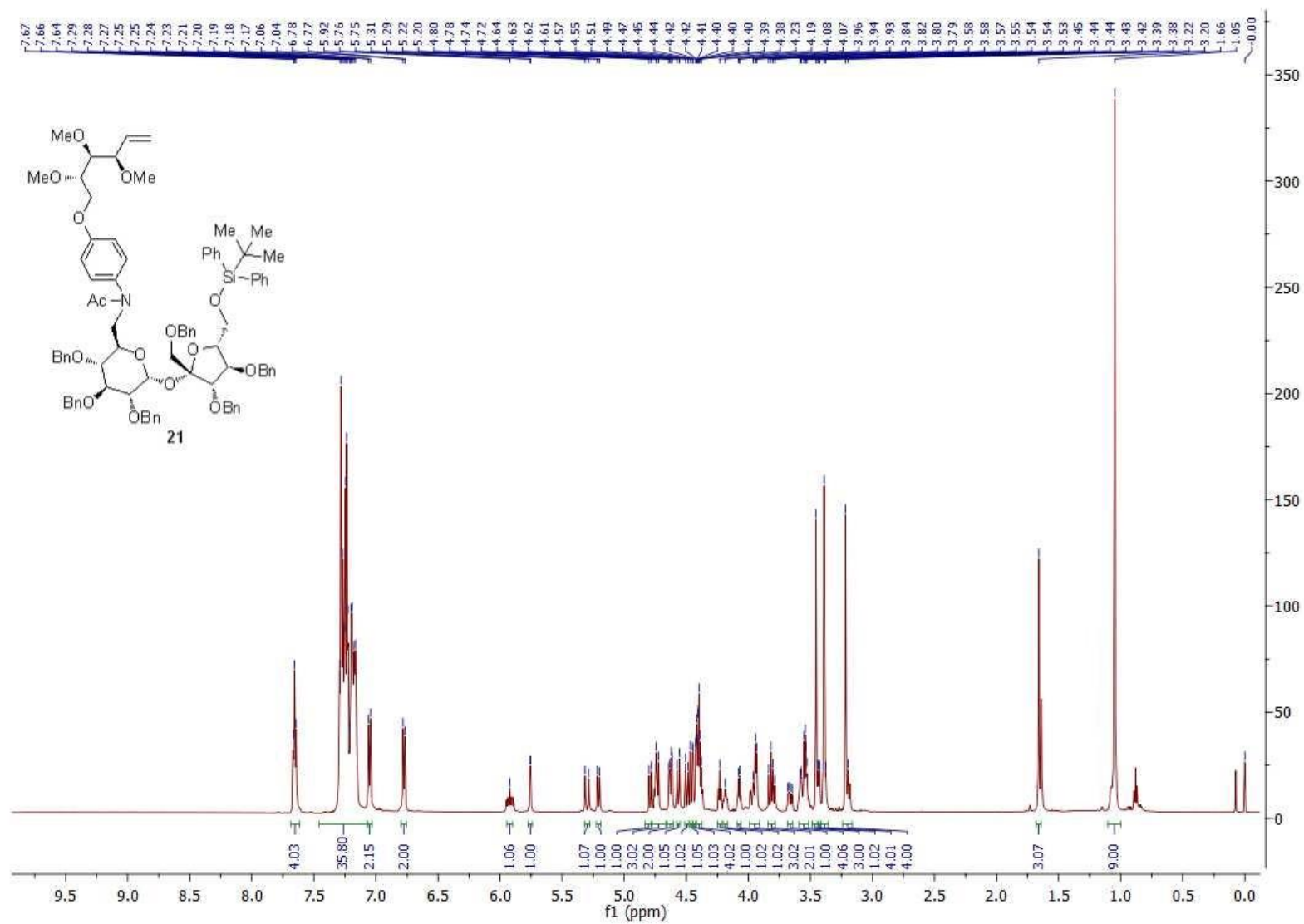
Figure S10 ^1\text{H} NMR spectrum of compound 21 .
