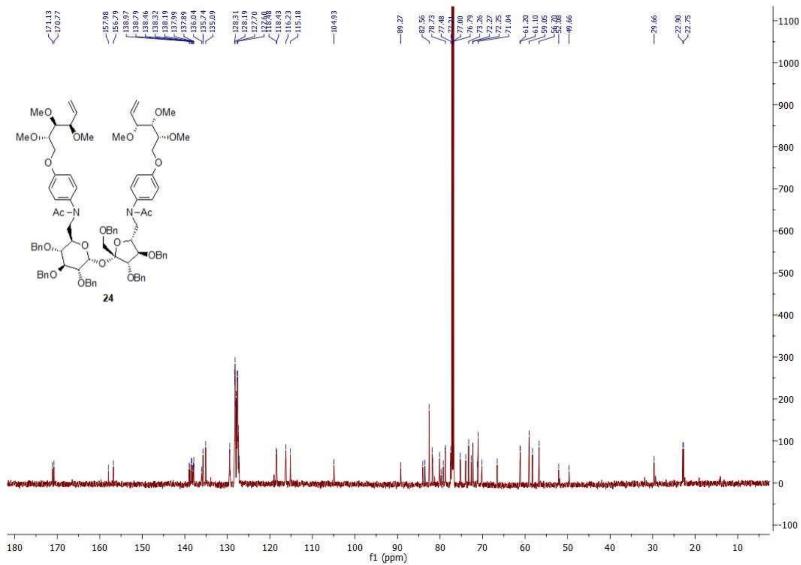
Figure S23 13 C NMR spectrum of compound 24 .
