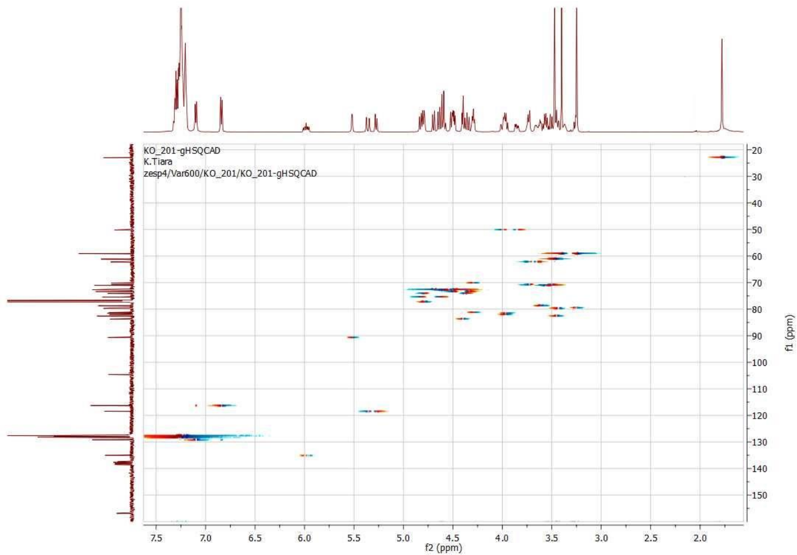
Figure S20 gHSQCAD spectrum of compound 22 .
