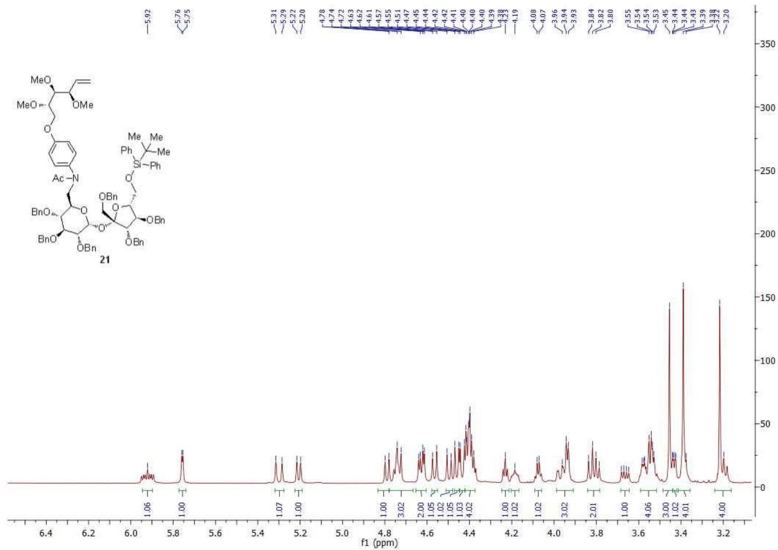
Figure S11 ^1\text{H} NMR spectrum (aliphatic part) of compound 21 .
