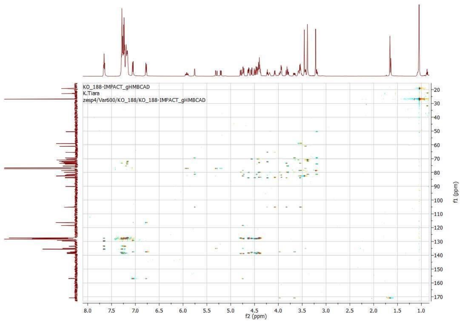
Figure S15 gHMBCAD spectrum of compound 21 .
