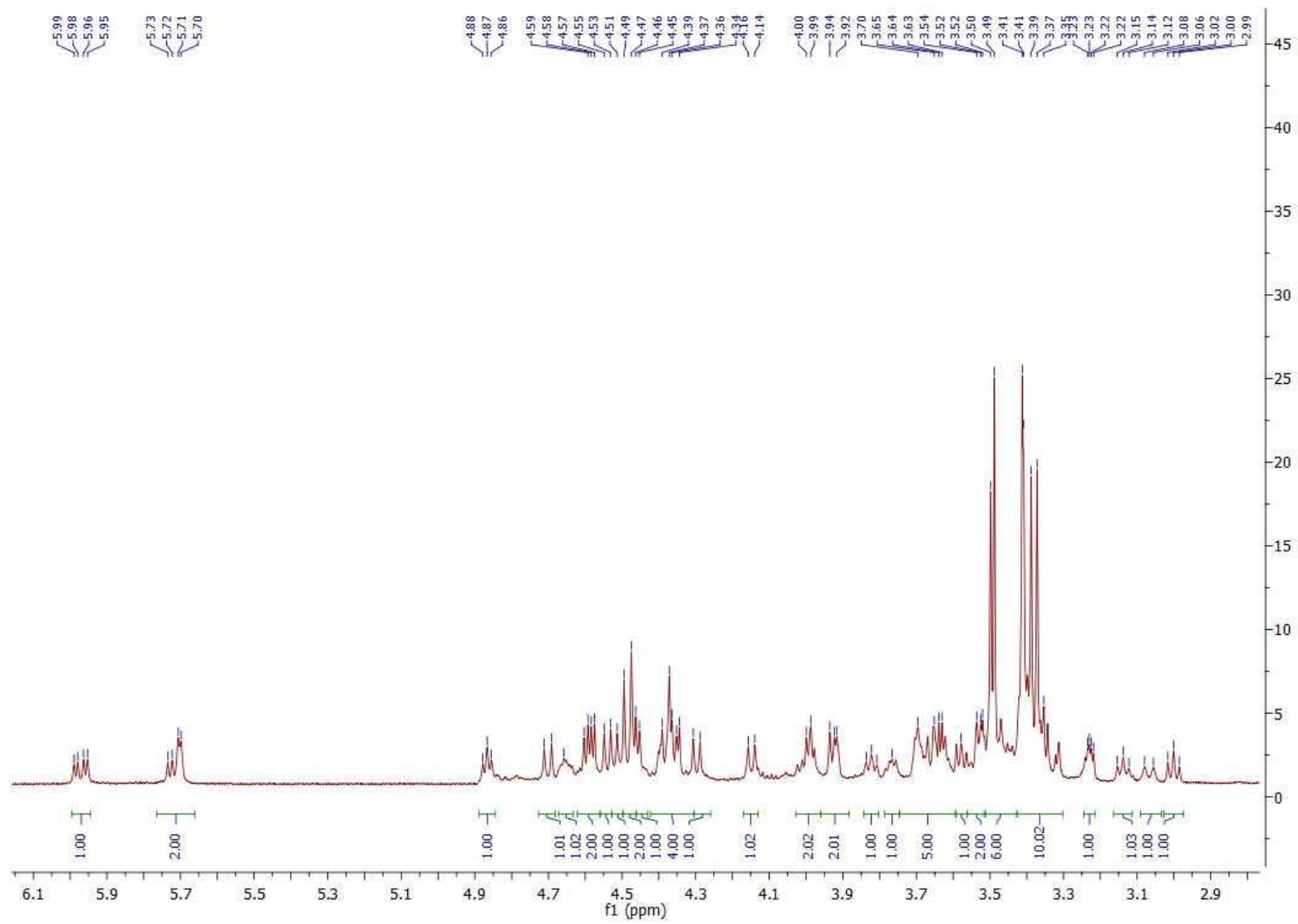
Figure S27 ^1\text{H} NMR spectrum (aliphatic part) of compound 25 .
