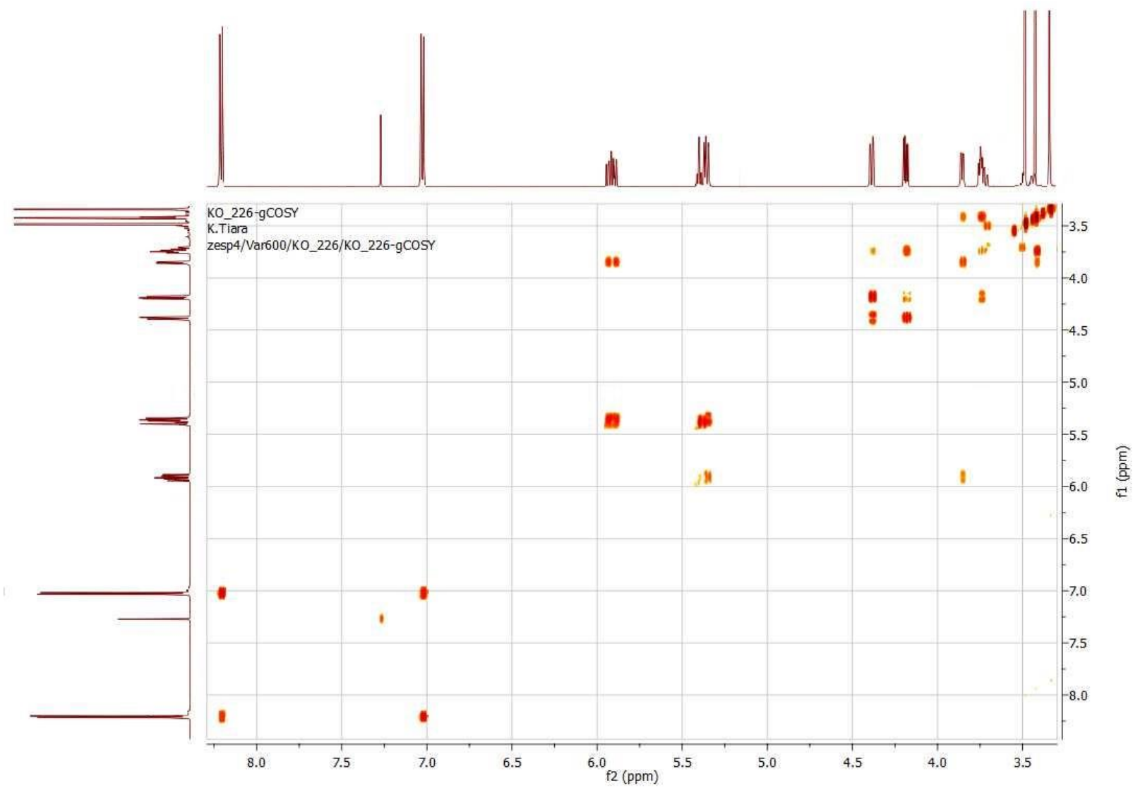
Figure S8 gCOSY spectrum of compound 16 .
