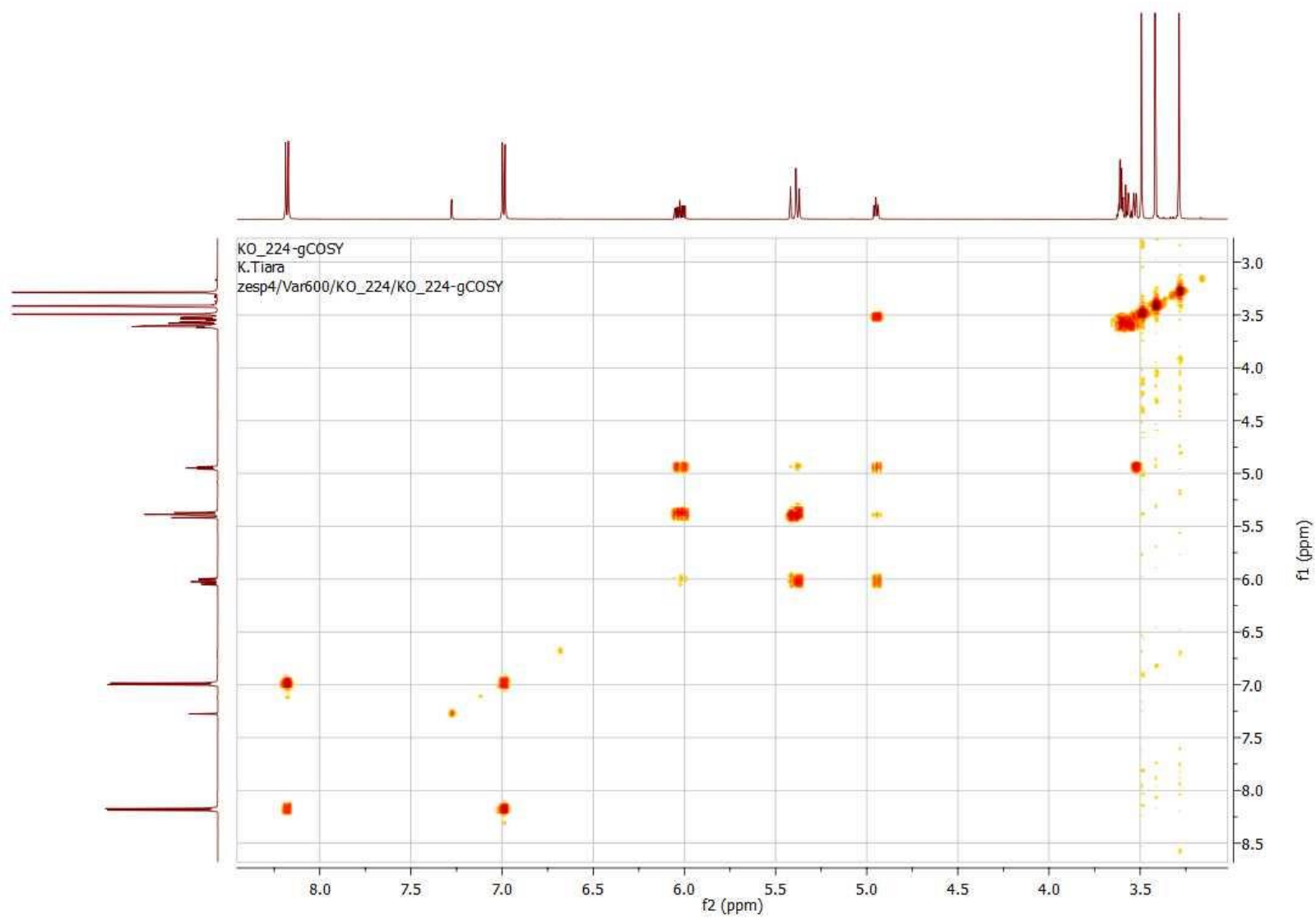
Figure S3 gCOSY spectrum of compound 14 .
