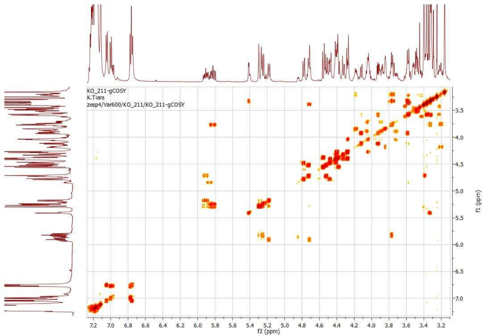
Figure S24 gCOSY NMR spectrum of compound 24 .
