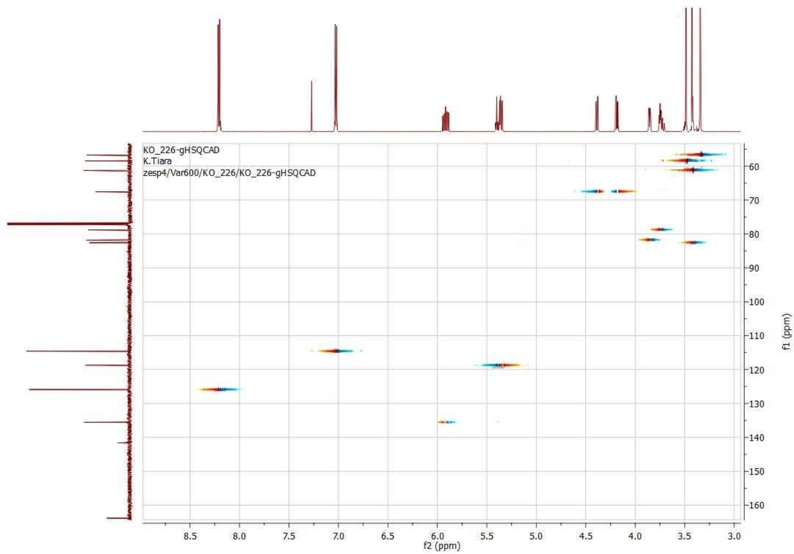
Figure S9 gHSQCAD spectrum of compound 16 .
