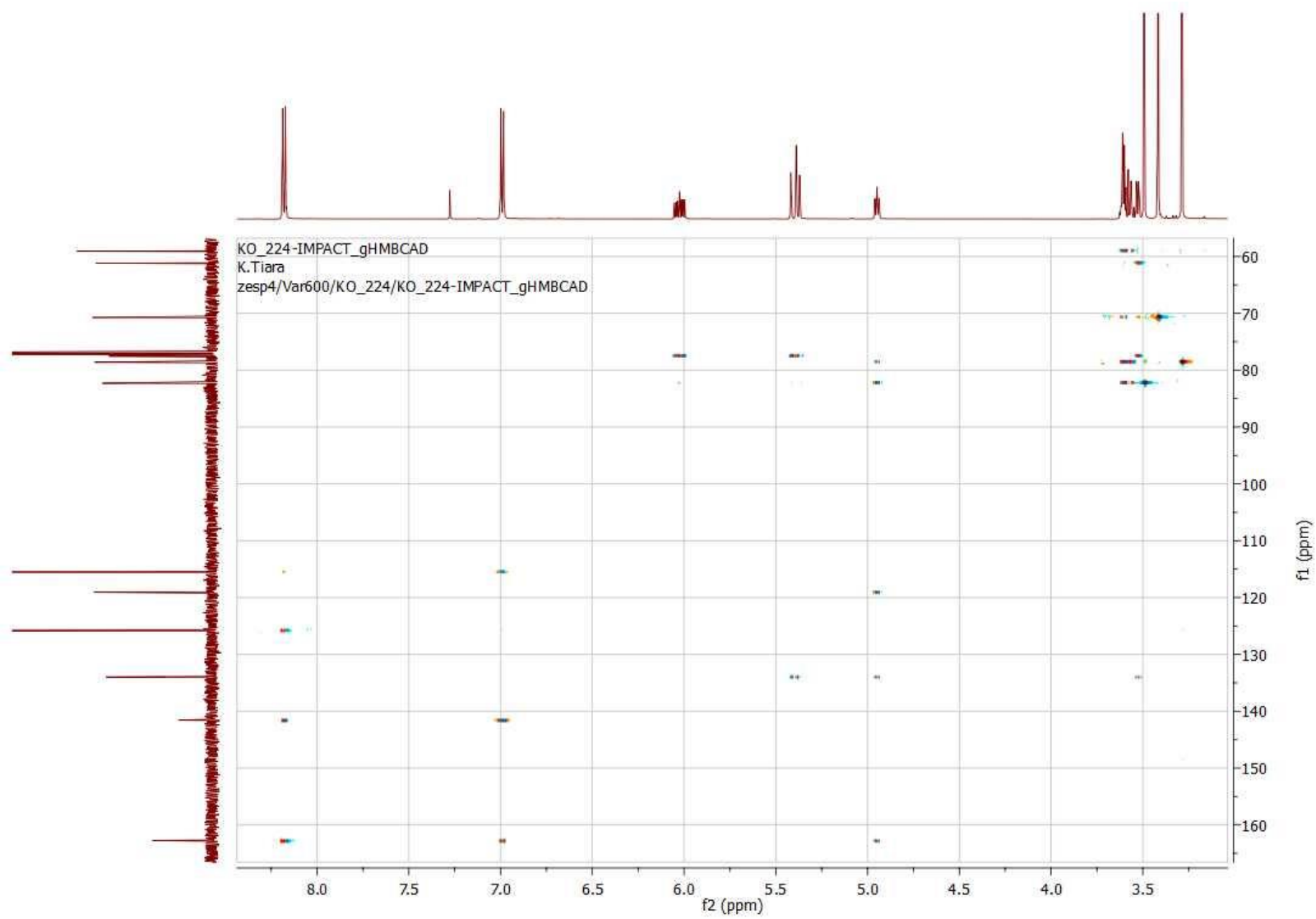
Figure S5 gHMBCAD spectrum of compound 14 .
