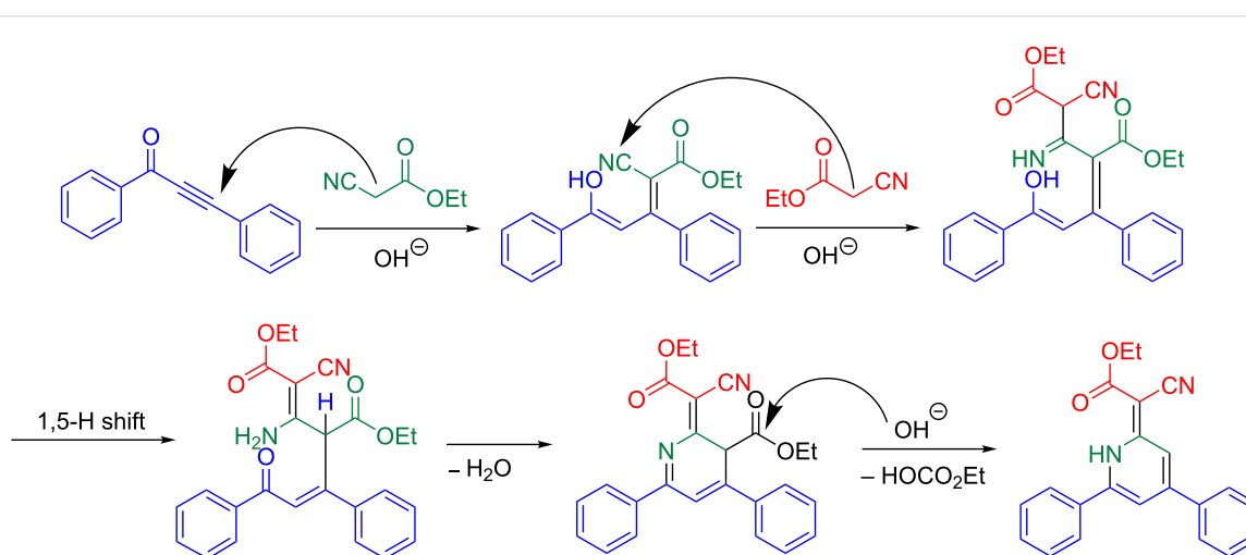
Scheme 9: Mechanistic rationale for the formation of the 1H -pyridine 5a .
