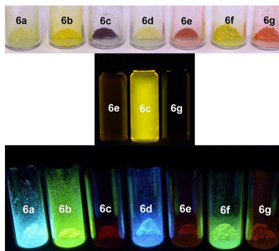
Figure 8: \alpha -Pyrones 6 as solids under daylight (top), selected derivatives under UV light ( \lambda_{\text{exc}} = 365 nm, c(\mathbf{6}) = 10^{-4} M) in dichloromethane solution (center), and under UV light ( \lambda_{\text{exc}} = 365 nm) in the solid state (bottom).
