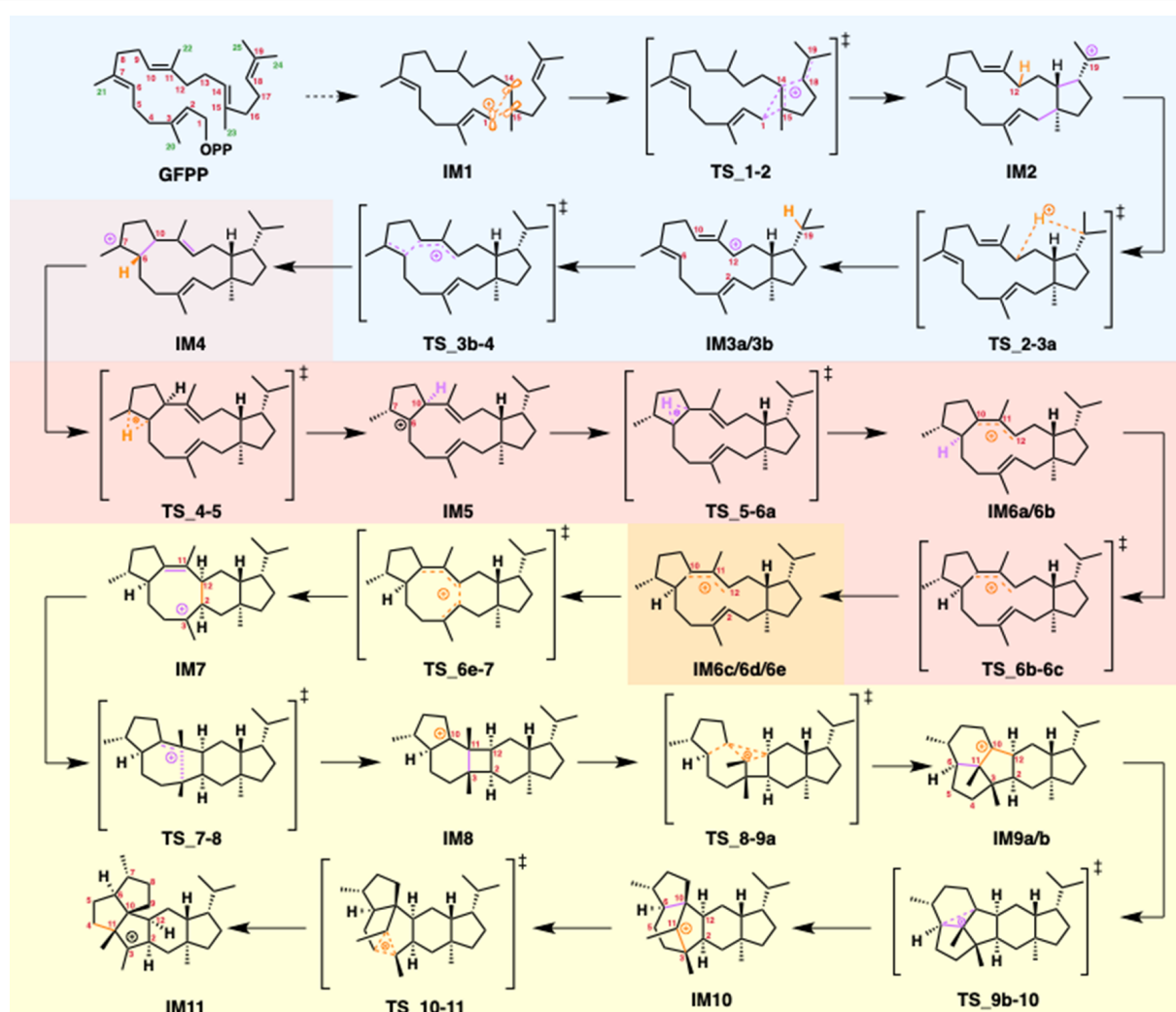
Scheme 2: Reaction mechanism of quinuclidine biosynthesis. GFPP: geranylarnesyl diphosphate, IM: intermediate. Quinuclidine is formed by the deprotonation of IM11 . Phase (I): 5/12/5 tricycle formation is highlighted in blue. Phase (II): conformational changes and hydrogen shifts are highlighted in orange. Phase (III): ring rearrangements are highlighted in yellow.
