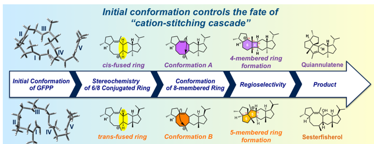
Scheme 1: The regio- and stereoselectivity in quinuclidine and sesterfisherol biosynthesis are determined by the initial conformation of GFPP.
