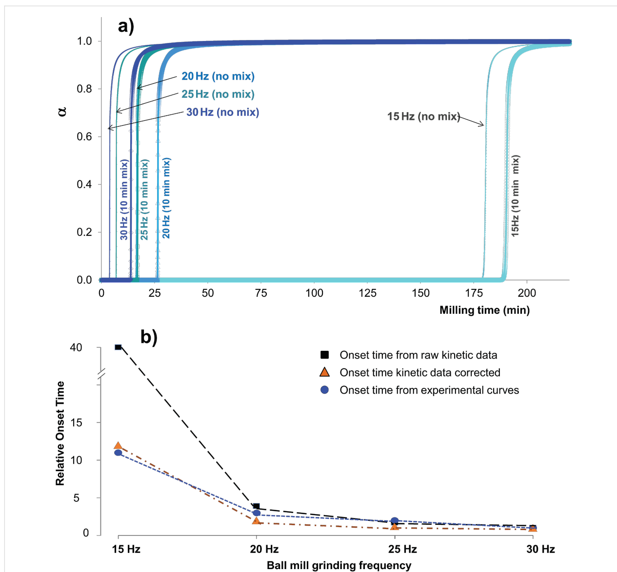
Figure 2: Reaction profiles for mechanochemical milling according to Equation 4. (a) Kinetic profiles for 30 Hz, 25 Hz, 20 Hz and 15 Hz NG milling. Raw (fine line curves) and corrected (base onset time + 10 min; thick line curves) are given and labelled. Onset time (normalized relative to 30 Hz model data) correction approximated from experimental curves. (b) Comparison of relative conversion onset times from raw kinetic curves (black rectangles), onset time corrected (brown triangles), and from experimental ball mill NG curves (blue circles) in Figure 1. E_0:\tau = 17.48 .
