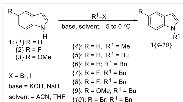
Scheme 3: Synthesis of the starting N -alkylindoles 1 {4–10}.
