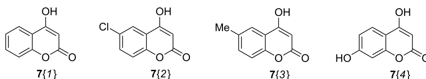
Scheme 5: Chemset of coumarins 7 {1–4} for elaboration in the MCR experiments.
