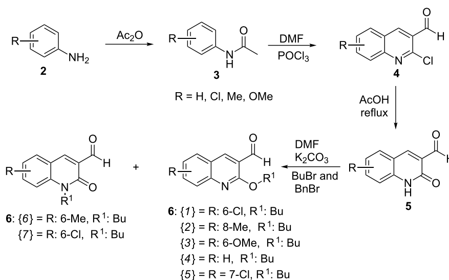
Scheme 4: General procedure for the synthesis of the starting quinoline/quinolone aldehydes 6 {1–7}.
