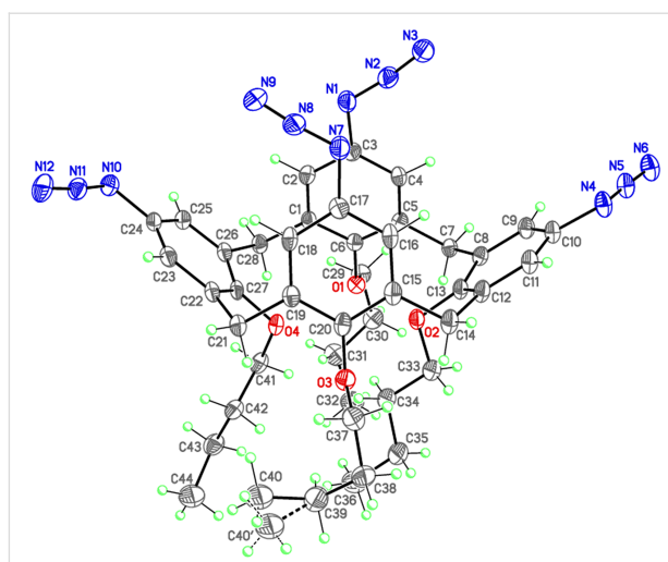
Figure 1: Molecular structure of 8a (50% ellipsoids). The dashed line indicates the alternative position of the disordered n -butyl group with the minor occupancy.
