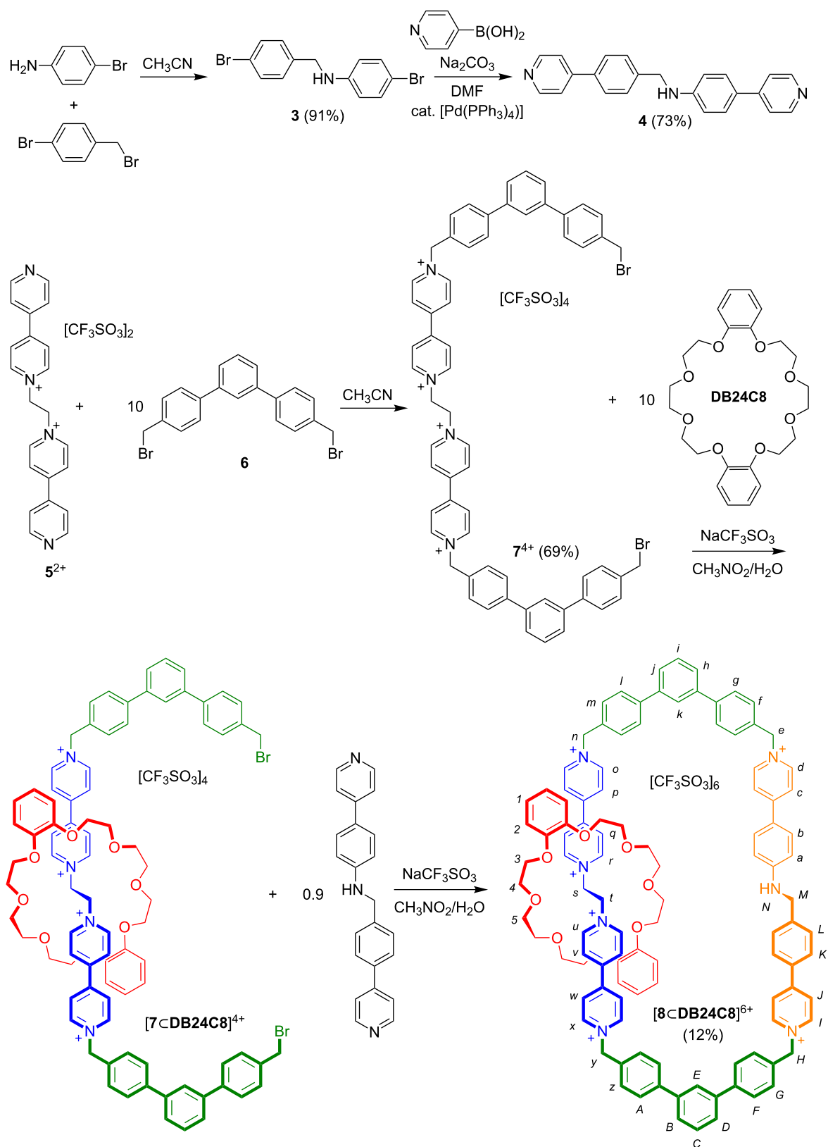
Scheme 1: Step-wise synthesis of [2]catenane [8<DB24C8>] 6+ containing benzylianium and bis(pyridinium)ethane recognition sites and terphenyl spacers.
