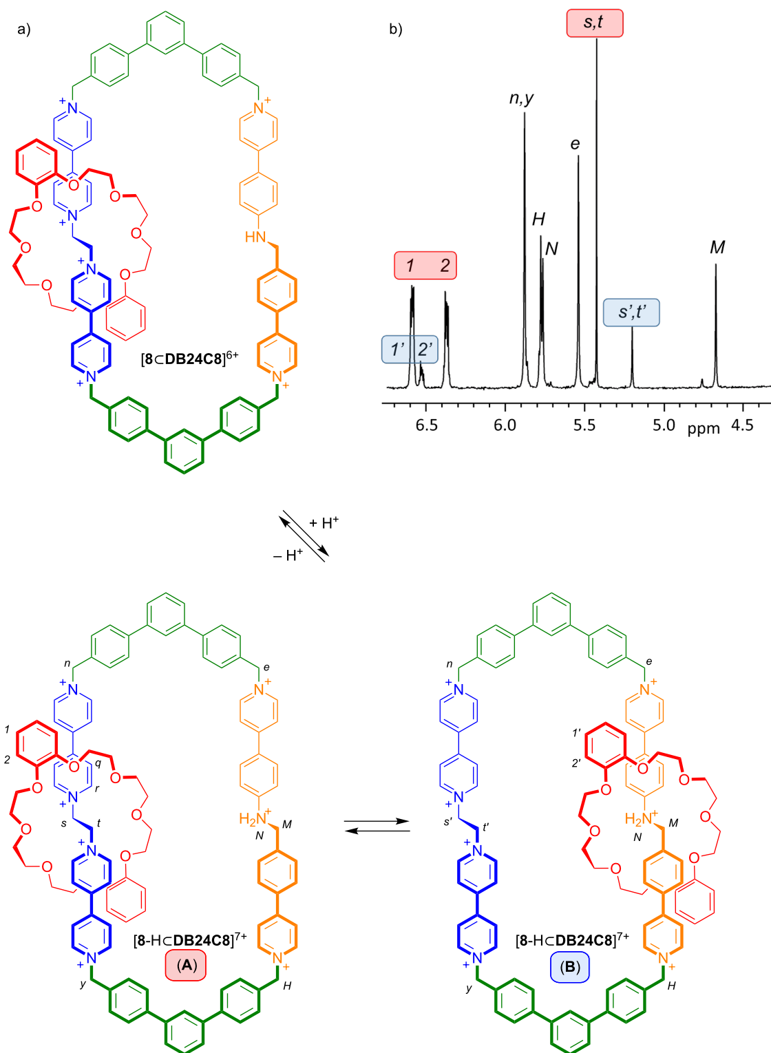
Figure 4: a) The [2]catenane [8CDB24C8]^{6+} can be protonated to yield [8-HCDB24C8]^{7+} in two different co-conformations A and B . b) The partial ^1H NMR spectrum (500 MHz, 298 K, CD_3CN ) of [8-HCDB24C8]^{7+} shows key resonances for both co-conformations A (red) and B (blue). See Scheme 1 for labelling; atoms of co-conformer B are labelled with a prime, e.g., s' versus s .
