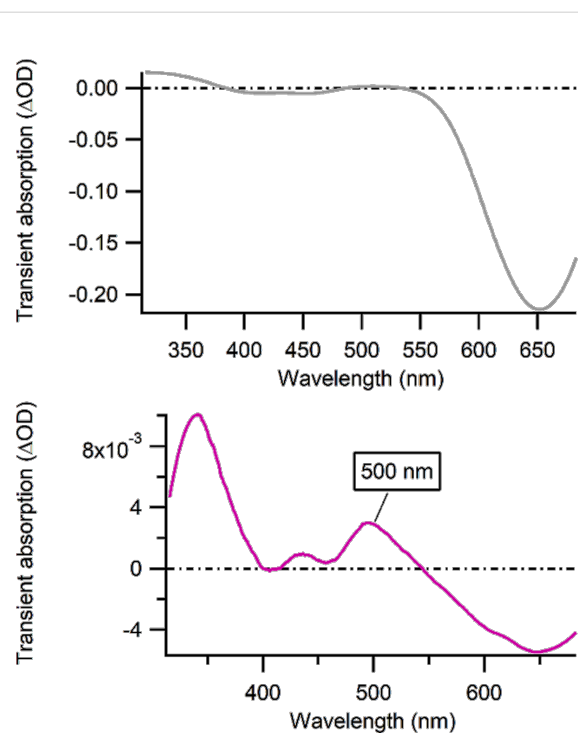
Figure 5: Transient absorption spectra of Ru II -calix[4]arene-[c-(RGDfK)] 4 conjugate 9 (in 10 mM Tris-HCl buffer at pH 7.0) measured 500 ns after the laser pulse (gray, top) and 1 μs after the laser pulse in the presence of 10 mM GMP (purple, bottom).
