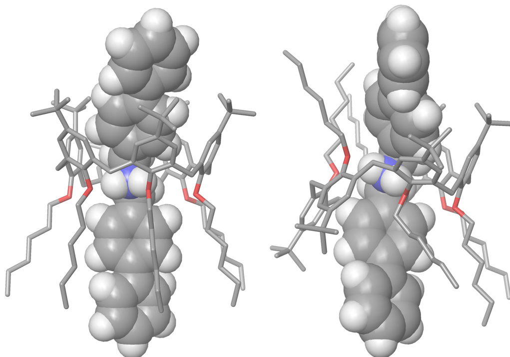
Figure 7: DFT-optimized structures of the: (left) 2^+ \subset \mathbf{1}^{\text{cone}} and (right) 2^+ \subset \mathbf{1}^{\text{1,2,3-alt}} pseudorotaxane atropoisomers calculated at B3LYP/6-31G(d,p) level of theory and using Grimme's dispersion corrections (IOP(3/124 = 3)).
