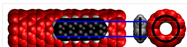
Figure 6: The contact zone of an (8,0)-CNT/tetracene complex. The bold black lines in the traverse section represent the positions of the nuclei. Reprinted with permission from [44], copyright 2017 Elsevier.
