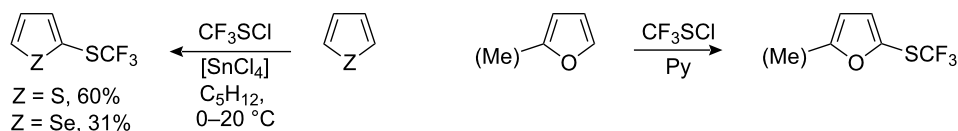
Scheme 17: Reactions of furan, thiophene and selenophene with \text{CF}_3\text{SCl} .
