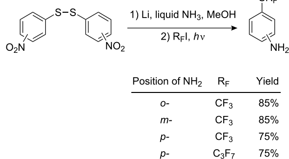
Scheme 40: Preparation of R F S-substituted anilines from dinitrothiophene disulfides.
