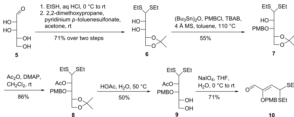
Scheme 2: Initial attempt on the synthesis of the C 4 aldehyde from D -lyxose ( 5 ).
