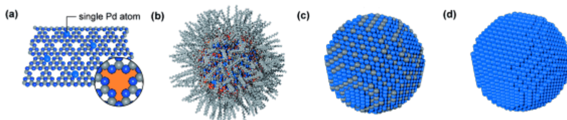
Figure 4: Structure of \text{Pd}@ \text{mpg-C3N4} (a), \text{Pd}(\text{HDMa})@ \text{C} (b), \text{Pd}(\text{Pb})@ \text{CaCO}_3 (c) and \text{Pd}@ \text{Al}_2\text{O}_3 (d) catalysts. The structures depict the increasing size of the active ensemble, from a single Pd atom (a) to a bare PdNP of approximately 800 atoms (d). The inset in (a) shows a characteristic six-fold cavity (orange) in the carbon nitride structure. C light grey, N dark blue, O red, Pb grey, Pd light blue. Adapted with permission from [122], © 2015 John Wiley and Sons.
