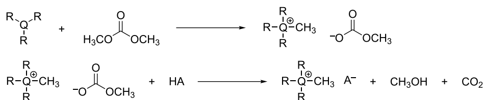
Scheme 3: Top: Green methylation of phosphines and amines by dimethyl carbonate ( Q = N, P ). Bottom: anion metathesis of methyl carbonate onium salts.
