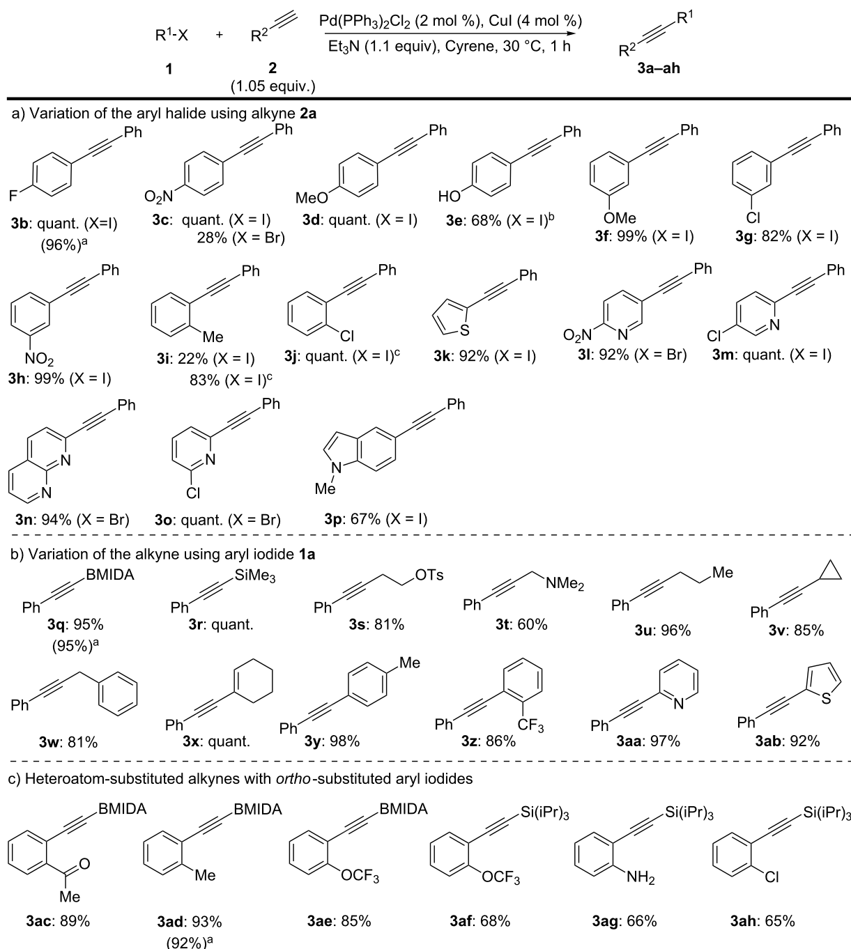
Scheme 2: Cyrene-based Sonogashira cross-coupling: Substrate scope. Isolated yields. a Yield using DMF as solvent. b 2 equiv of Et 3 N used. c 24 h reaction time.
