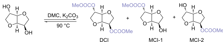
Scheme 3: Methoxycarbonylation of isosorbide via DMC chemistry.
