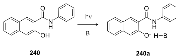
Figure 170: Anion sensor principle with 3-hydroxy-2-naphthalenylidene of Jiang et al.
