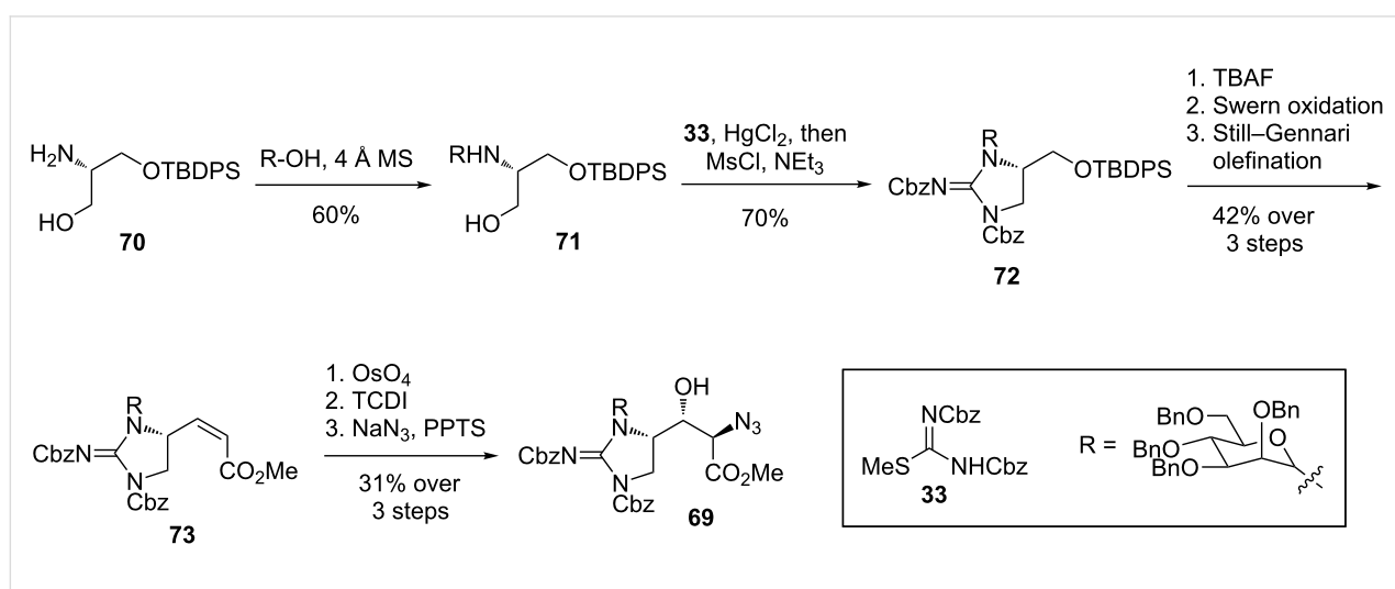
Scheme 13: Synthesis of \beta -hydroxyenduracididine derivative 69 .
