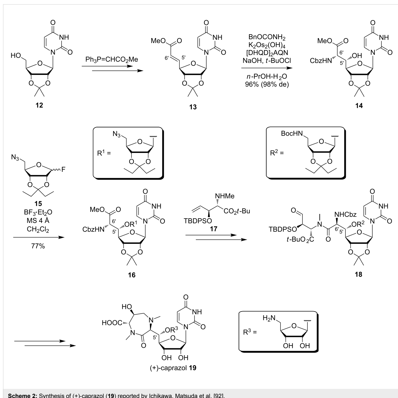
Scheme 2: Synthesis of (+)-caprazol ( 19 ) reported by Ichikawa, Matsuda et al. [92].
