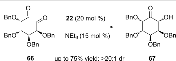
Scheme 40: Intramolecular benzoin condensation of carbohydrate-derived dialdehydes.
