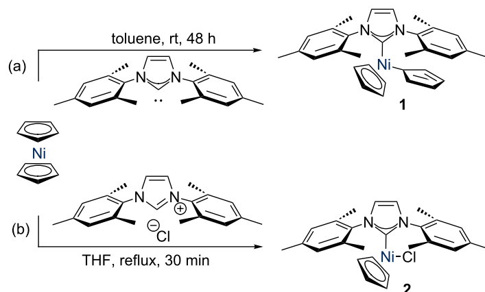
Scheme 1: Synthesis of [Ni(η 1 -Cp)(η 5 -Cp)(IMes)] ( 1 ) and [NiCl(Cp)(IMes)] ( 2 ).
