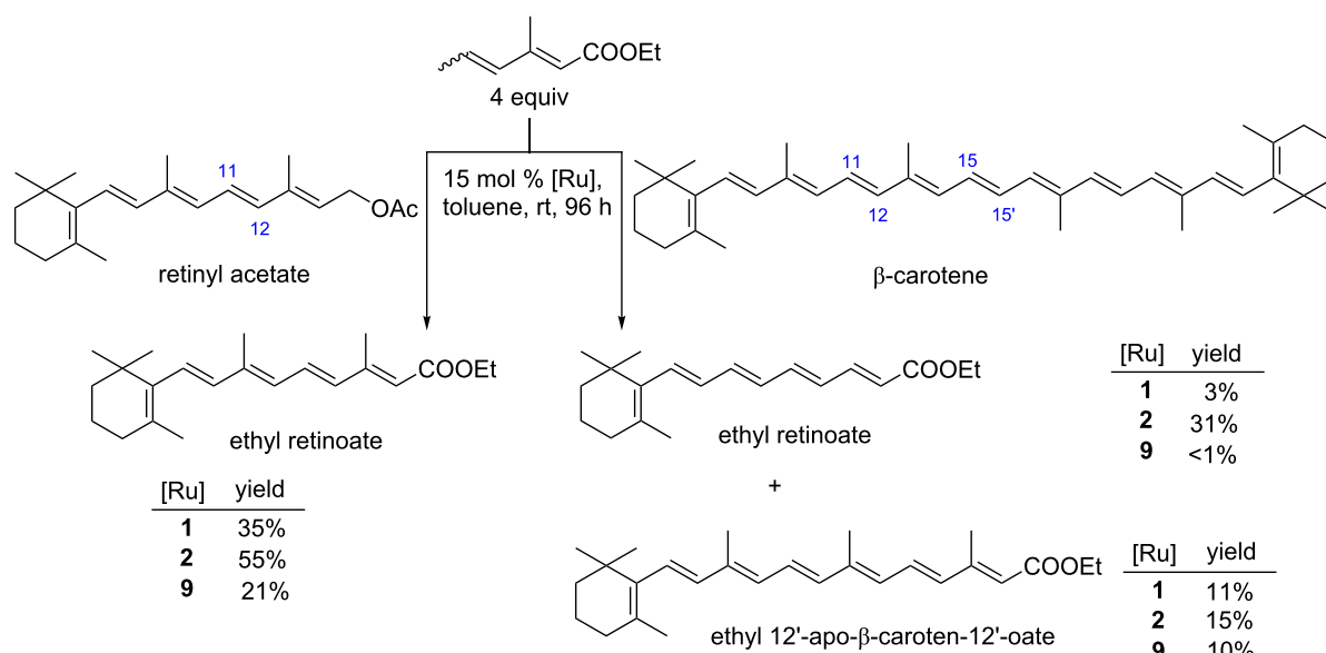
Scheme 4: CM reaction of \beta -carotene and retinyl acetate with ethyl (2 E ,4 Z/E )-3-methylhexa-2,4-dienoate. Reaction conditions: diene (4 equiv, 0.325 M), alkene (1 equiv, 0.08 M). Yield was obtained by quantitative HPLC analysis. Yields were calculated in relation to polyene (retinyl acetate or \beta -carotene). In case of the \beta -carotene reaction, yields were divided by two due to the symmetry of the \beta -carotene molecule.
