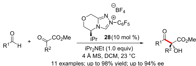
Scheme 15: Enantioselective cross-benzoin reactions of aliphatic aldehydes and \alpha -ketoesters.
