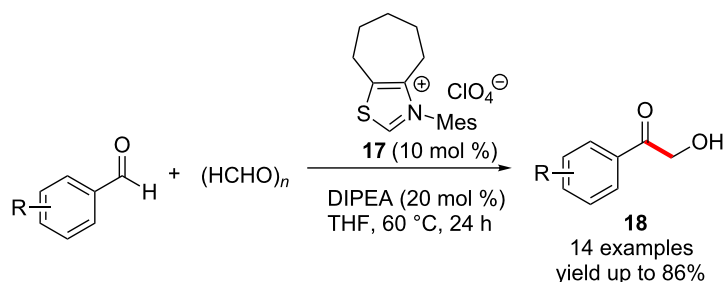
Scheme 8: Cross-benzoin reactions catalysed by thiazolium salt 17 .
