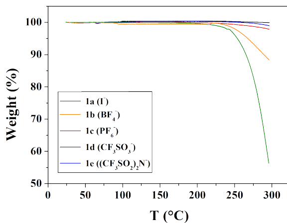
Figure 4: TGA measurements of the compounds 1a-e (rate 10 °C·min -1 , in air).
