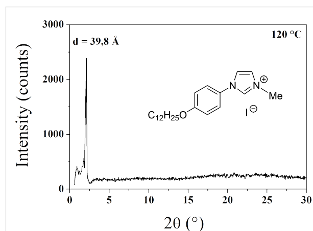
Figure 6: Powder X-ray diffraction pattern of compound 1a in the liquid crystal state ( T = 120 \text{ °C} ).
