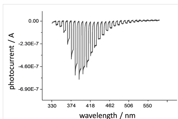
Figure 6: Photocurrent generated at the [\text{CrF}_5(\text{H}_2\text{O})]^{2-}@TiO_2 electrode as a function of the wavelength of the incident light, recorded at constant potential of 500 mV vs Ag/AgCl. The spikes originate from the opening and closing of the shutter.
