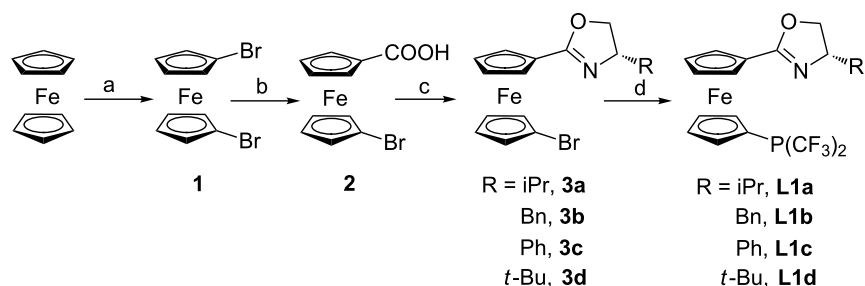
Scheme 2: Preparation of 1-[bis(trifluoromethyl)phosphino]-1'-oxazolinyloxyferrocene ligands. Reagents and conditions: (a) (i) n -BuLi, TMEDA, Et 2 O, rt; (ii) (BrCF 2 ) 2 , -78 °C. (b) n -BuLi, CO 2 , THF, -20 °C. (c) (i) (COCl) 2 , DCM, rt; then TEA, amino alcohol, DCM, rt; (ii) Ph 3 P, CCl 4 , TEA, CH 3 CN, rt. (d) (i) n -BuLi, TMEDA, P(OPh) 3 , Et 2 O, -78 °C; (ii) TMSCF 3 , CsF, Et 2 O, rt.
