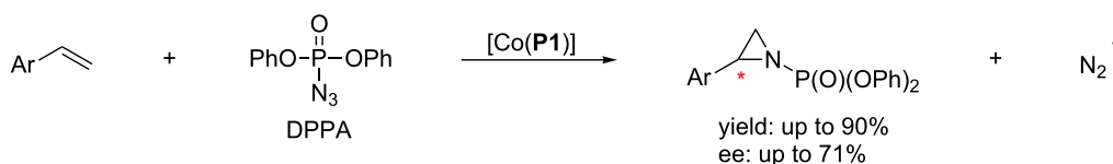
Scheme 2: [Co( P1 )]-catalyzed asymmetric olefin aziridination with DPPA.
