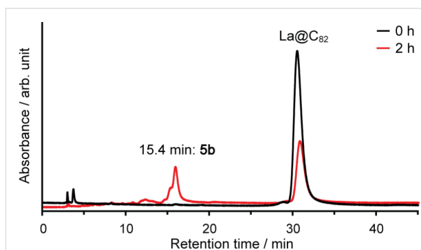
Figure 10: HPLC profiles of the reaction mixture for 5b . Conditions: column, Buckyprep ( \varnothing 4.6 mm \times 250 mm); eluent, toluene; flow rate, 1.0 mL/min; wavelength: 330 nm; 40 ^\circ\text{C} .
