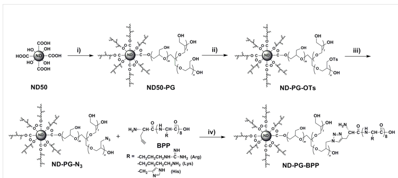
Scheme 1: Synthetic route from ND50 to ND-PG-BPP; i) glycidol, 140 °C, 20 h; ii) p -TsCl, pyridine, 0 °C to rt; iii) NaN 3 , 90 °C, overnight; iv) copper(II) sulfate pentahydrate, sodium ascorbate, rt, 96 h.
