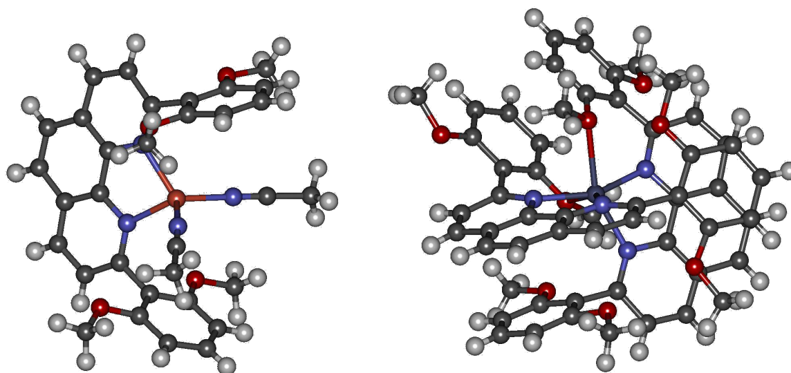
Figure 5: X-ray crystal structure analysis of [\text{Cu}(\text{H}_3\text{CCN})_2(\mathbf{22})]\text{BF}_4 and [\text{Zn}(\mathbf{22})_2](\text{OTf})_2 (counterions are omitted, colour code: orange: copper, petrol: zinc, grey: carbon, red: oxygen, blue: nitrogen, white: hydrogen).
