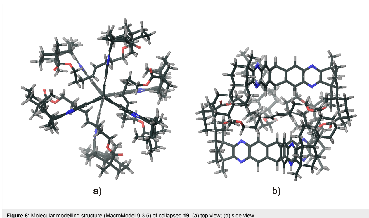
Figure 8: Molecular modelling structure (MacroModel 9.3.5) of collapsed 19 , (a) top view; (b) side view.
