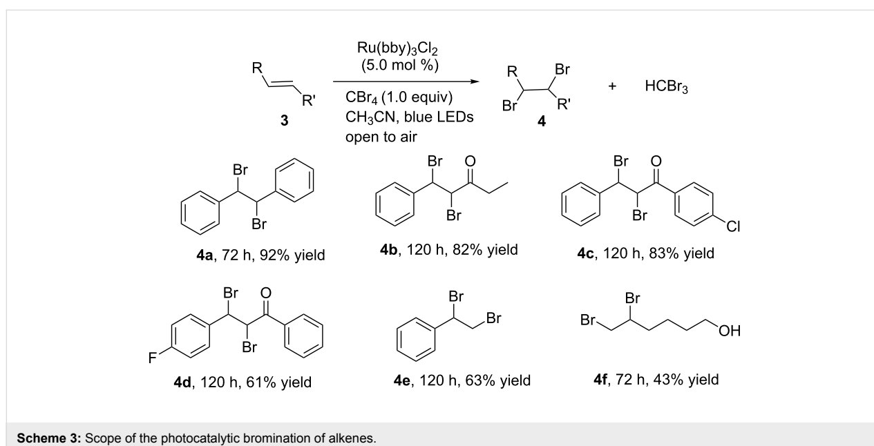
Scheme 3: Scope of the photocatalytic bromination of alkenes.
