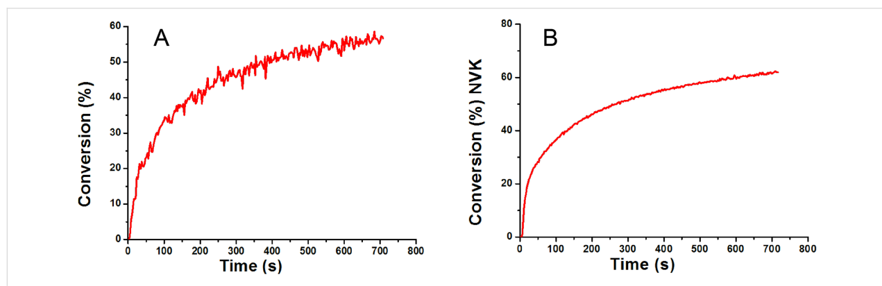
Figure 10: (A) Photopolymerization profile of EPOX; photoinitiating system: \text{Ir}(\text{piq})_2(\text{tmd})/\text{Ph}_2\text{I}^+/\text{NVK} (1%/2%/3%); laser diode at 532 nm exposure ( \sim 100 mW/cm ^2 ); under air. (B) Conversion profile for the NVK double bond in the course of the polymerization.
