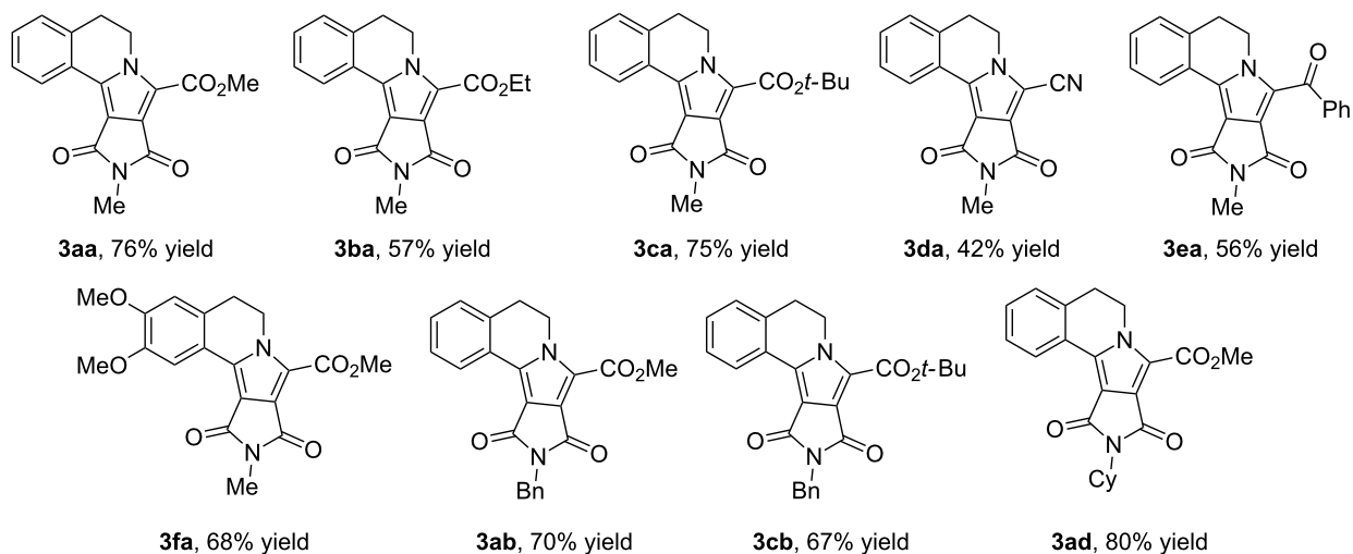
Scheme 2: Evaluation of the substrate scope.
