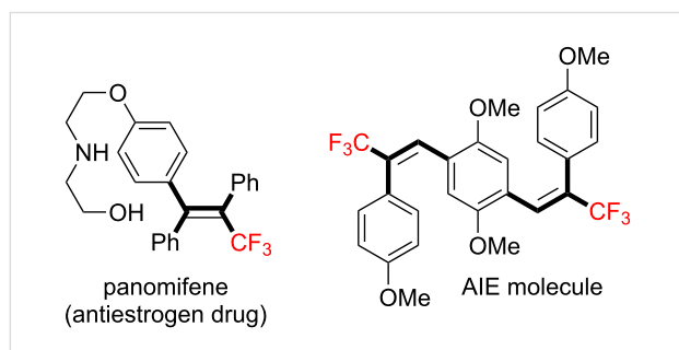
Scheme 1: Representative examples of multisubstituted \text{CF}_3 -alkenes.
