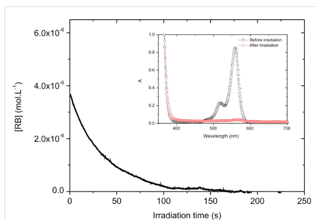
Figure 1: Evolution of RB concentration as a function of irradiation time ( \lambda = 532 \text{ nm} , 9 \text{ mW}\cdot\text{cm}^{-2} ); insert: absorption spectra obtained before and after irradiation.
