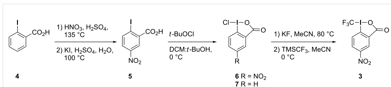
Scheme 1: Synthesis of 5-nitro-1-(trifluoromethyl)-3 H -1 \lambda^3 ,2-benziodaoxol-3-one ( 3 ).
