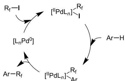
Figure 3: Plausible catalytic cycle proposed by M. S. Sanford et al. for the perfluoroalkylation of simple arenes using perfluoroalkyl iodides [70].
