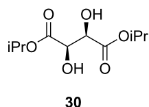
Figure 3: Diisopropyl L-tartrate ( 30 ) used as a chiral modifier for NMR determination of ee.
