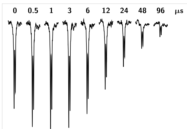
Figure 3: Time-resolved CIDNP signals of the 18 equivalent \beta protons ( d , 0.98 ppm) of triisopropylamine (TIPA) in the photoreaction with xanthone (XA) as functions of the delay (given at the respective trace) between the laser flash and the sampling NMR pulse. Note the exponential increase of the delay with the spectrum number. Excitation intensity, ca. 80 mJ per flash; NMR pulse width, 1.0 \mu s; temperature, 279 K; amine concentration, 5.0 \times 10^{-4} M; sensitizer concentration, 1 \times 10^{-3} M. Further explanation, see text.
