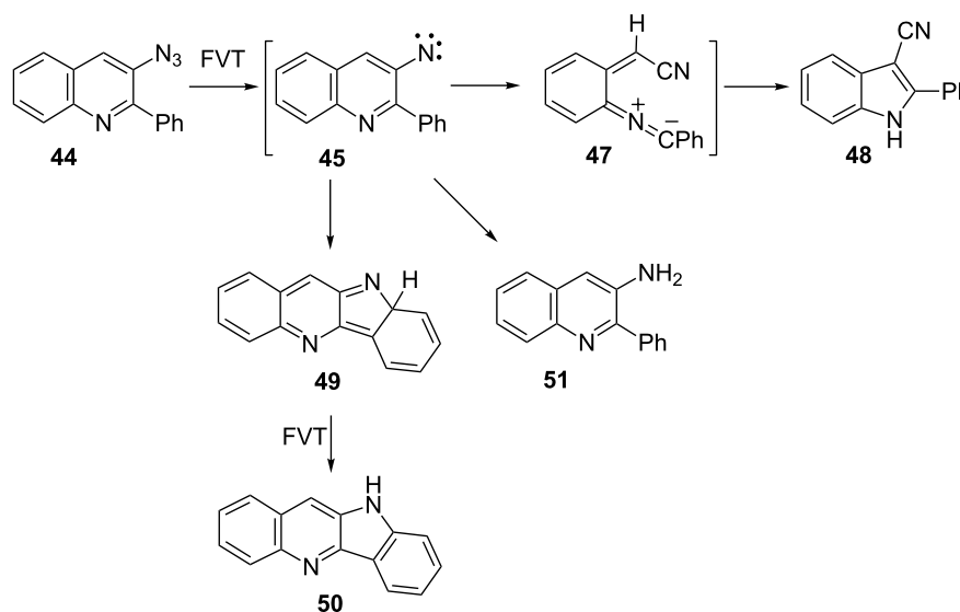
Scheme 12: Preparative FVT of 3-azido-2-phenylquinoline.
