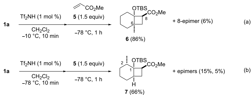
Scheme 2: Regioselective formation of bicyclo[4.2.0]octanes from the same substrates by the isomerization–(2 + 2) cycloaddition procedure.
