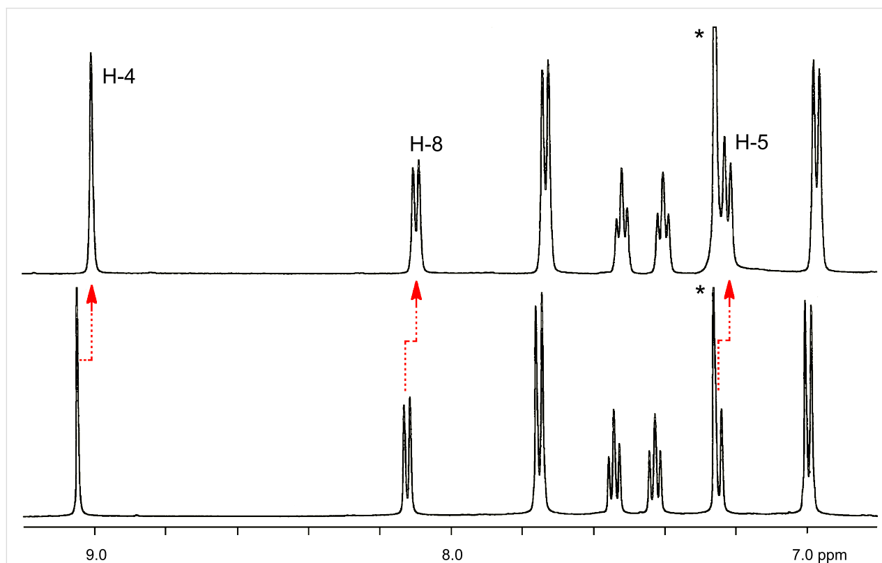
Figure 4: Aromatic region of the 1 H NMR ( CDCl_3 , 500 MHz, 25 °C) spectra of macrocycle ( R,R )- 12 (2.8 mM, bottom) and at the end of the titration with tetrabutylammonium succinate ( [(R)-7] = 2.8 mM, [(CH_2CO_2)_2(Bu_4N)_2] = 28 mM, top). Asterisks indicate the residual solvent peaks.
