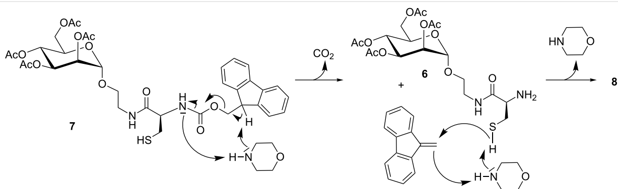
Scheme 3: Proposed mechanism for the formation of S -Fmoc-protected 8 from N -Fmoc-protected 7 according to Rich and co-workers [16].
