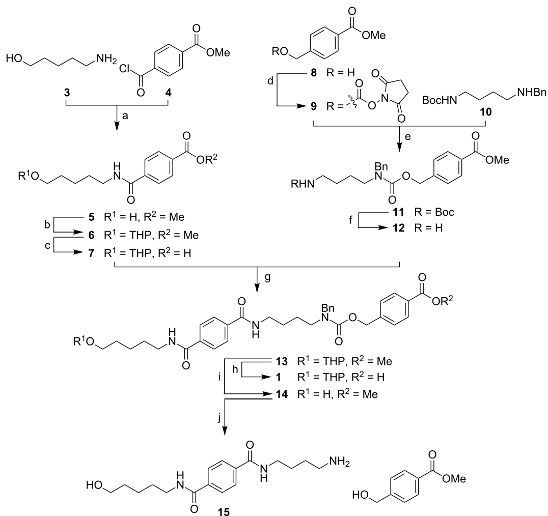
Scheme 3: Synthesis of linker 1 . Reactions and conditions: (a) NEt_3 , DCM, rt, 84%; (b) DHP, pyridinium p -toluenesulfonate, DCM, rt, quant.; (c) 2 M aq NaOH, THF, rt, 91%; (d) DSC, NEt_3 , CH_3CN , 0 °C to rt; (e) NEt_3 , DCM, rt, 80% over 2 steps; (f) TFA, DCM, rt, 99%; (g) NHS, DCC, DMAP, CH_3CN , DCM, rt, 63%; (h) 2 M aq NaOH, THF, 55 °C, 92%; (i) p -TsOH· H_2O , MeOH, DCM, rt, 94%; (j) Pd(OAc)_2 , HCOONH_4 , MeOH, H_2O , 90%.
