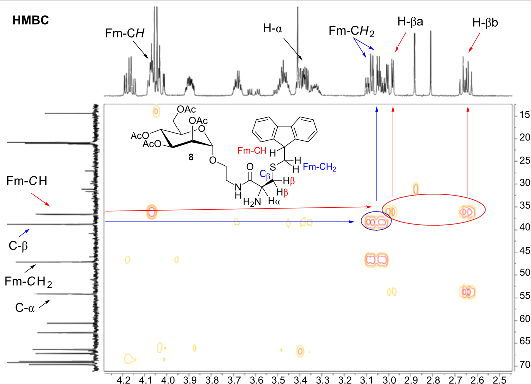
Figure 1: In the ^1\text{H}/^{13}\text{C} HMBC NMR spectrum of the S -Fm-protected glycoamino acid derivative 8 , protecting-group rearrangement is confirmed by the cross peaks between C-β and the Fm-CH 2 protons (in blue) and between Fm-CH and the H-β a ,β protons (in red).
