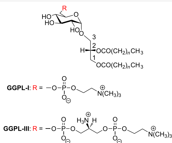
Figure 1: Absolute chemical structures of M. fermentans \alpha -glycolipid antigens, GGPI-I and GGPI-III (GGPI: Glycosyl- sn -glycerophospholipid).
