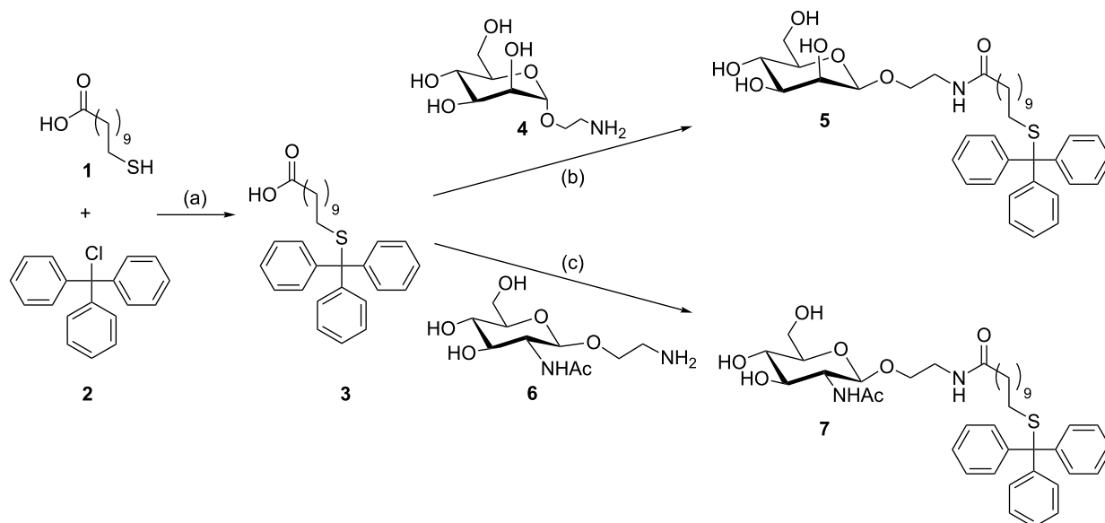
Scheme 1: Synthesis of the tritylated compounds 3 [28], 5 and 7 : (a) dichloromethane, 2.5 h, rt, 98%, (b) HBTU/DIPEA, dry DMF, overnight, rt, 74%, (c) HATU/DIPEA, dry DMF, 3 h, rt, 71%.
