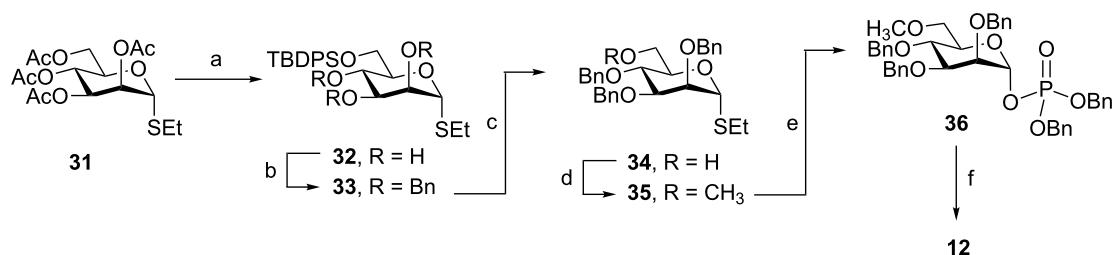
Scheme 4: Reagents and conditions: (a) (i) \text{NaOCH}_3 , \text{CH}_3\text{OH} ; (ii) \text{TBDPSCI} , imidazole, DMF, 78%; (b) \text{BnBr} , \text{NaH} , TBAI, 84%; (c) TBAF, THF, 83%; (d) \text{CH}_3\text{I} , \text{NaH} , DMF, 87%; (e) \text{HO-P(O)(OBn)}_2 , NIS, \text{AgOTf} , \text{CH}_2\text{Cl}_2 , 70%; (f) \text{H}_2 , \text{Pd(OH)}_2\text{-C} , \text{NaHCO}_3 , \text{CH}_3\text{OH} , 91%.
