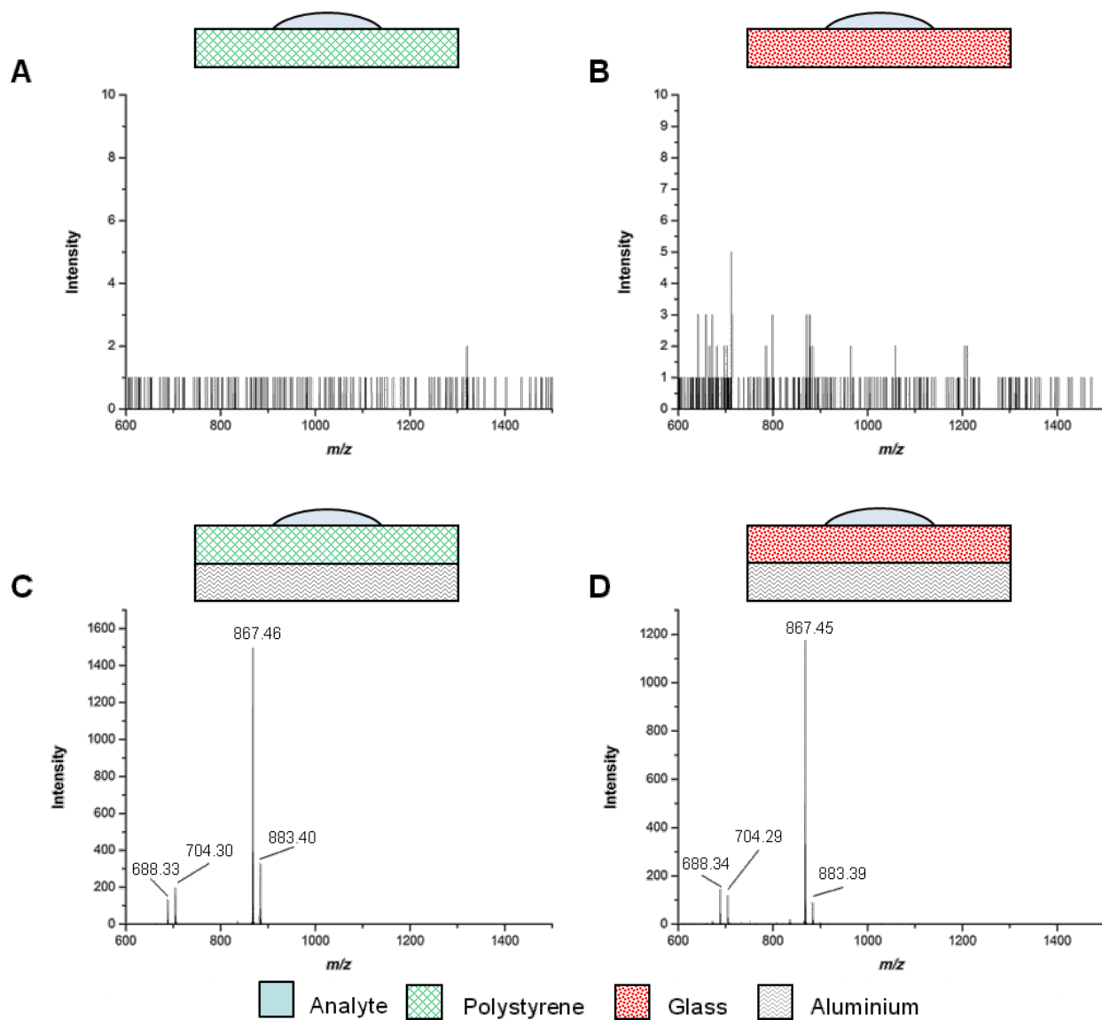
Figure 2: Comparison of the polystyrene and glass surfaces with and without aluminium backing by matrix-free MALDI-TOF MS analysis. Each spot contains 15 nmol Man-Trt ( 5 ): (A) polystyrene without aluminium; (B) glass without aluminium; (C) polystyrene with aluminium and (D) glass with aluminium. The peaks at m/z of 688.3, 704.3, 867.5 and 883.4 correspond to [\mathbf{5} + \text{Na}]^+ , [\mathbf{5} + \text{K}]^+ , [\mathbf{8} + \text{Na}]^+ , and [\mathbf{8} + \text{K}]^+ , respectively.
