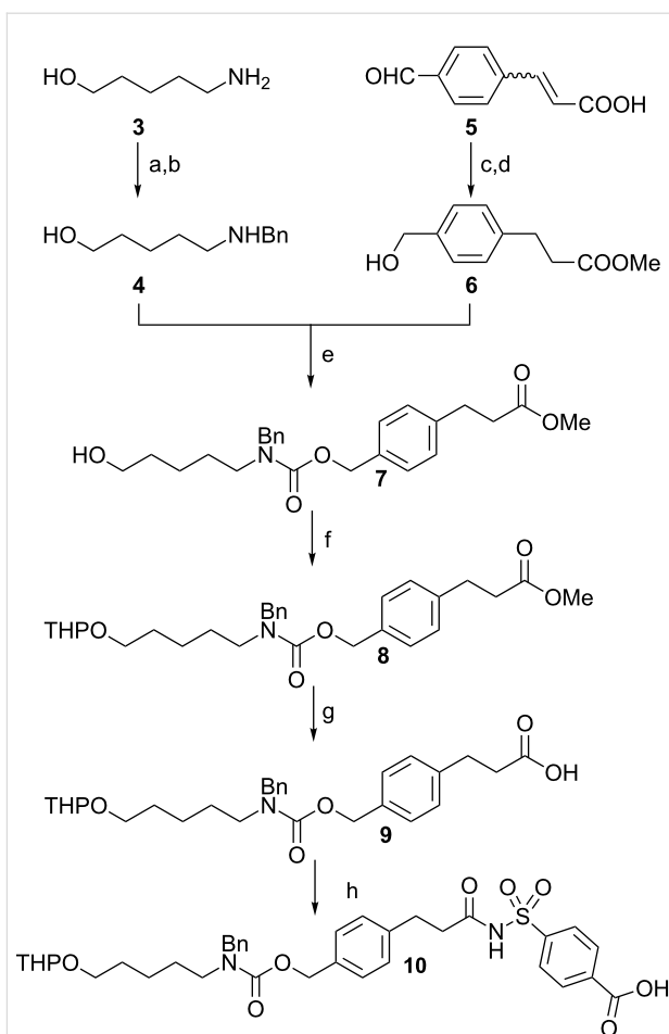
Scheme 1: Synthesis of a new acylsulfonamide safety-catch linker. Reagents and conditions: (a) benzaldehyde, \text{Na}_2\text{SO}_4 , DCM; (b) \text{NaBH}_4 , EtOH; 82% over two steps; (c) \text{H}_2 , 10% Pd/C, EtOH, DIPEA; (d) cat. \text{H}_2\text{SO}_4 , MeOH, 88% over two steps; (e) DSC, \text{Et}_3\text{N} , DCM/ \text{CH}_3\text{CN} , 85%; (f) DHP, p\text{-TsOH}\cdot\text{H}_2\text{O} , DCM, 86%; (g) \text{LiOH}\cdot\text{H}_2\text{O} , THF/ \text{H}_2\text{O} , reflux, 95%; (h) 4-sulfamoylbenzoic acid, DCC, DMAP, DCM/DMF, 60%.
