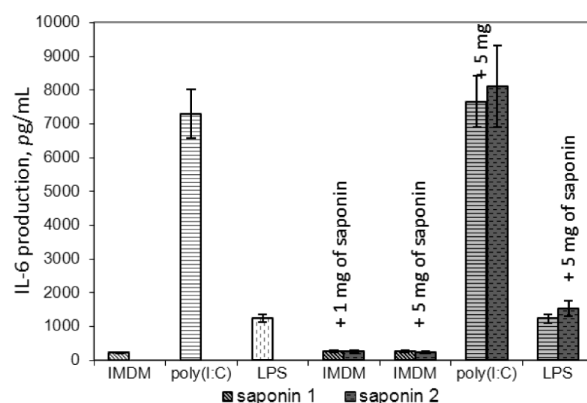
Figure 5: IL-6 production of primary endothelial cells in the presence of compounds 1 and 2 . Error bars represent the standard deviation in each point.
