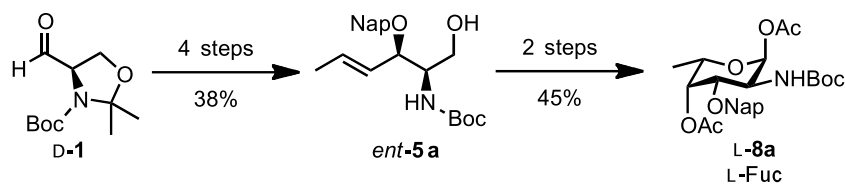
Scheme 5: Synthesis of L-fucosamine building block L-8a from D-Garner aldehyde.
