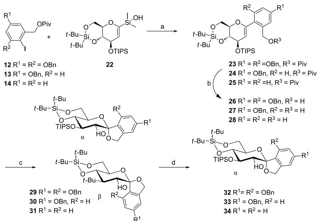
Scheme 3: (a) \text{Pd}_2(\text{dba})_3 \cdot \text{CHCl}_3 , NaOt-Bu, toluene, 50^\circ\text{C} , 6–20 h, 23 : 72%, 24 : 79%, 25 : 62%; (b) DIBAL-H, \text{CH}_2\text{Cl}_2 , -78^\circ\text{C} to rt, 0.5–1 h, 26 : 86%, 27 : 70%, 28 : 75%; (c) m -CPBA, \text{NaHCO}_3 , \text{CH}_2\text{Cl}_2 , 0^\circ\text{C} to rt, 2–2.5 h; (d) HCl, \text{CHCl}_3 , rt, 1 h, 32 : 91% over two steps, 33 : 83% over two steps, 34 : 86% over two steps.
