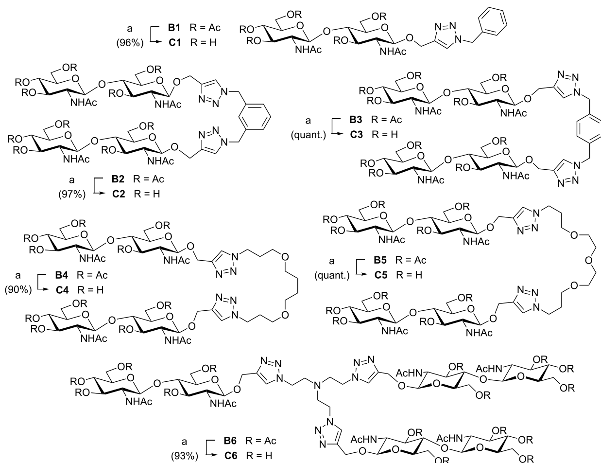
Scheme 2: Deacetylation of glycoconjugates B1–B6 . (a) NaOMe, MeOH.
