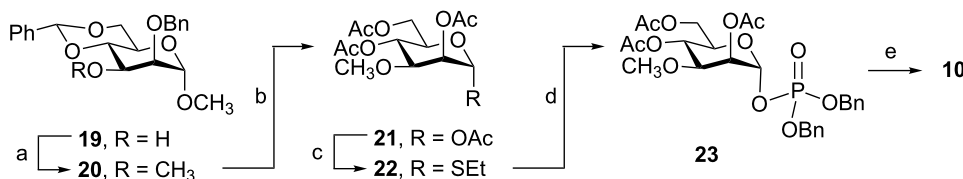
Scheme 2: Reagents and conditions: (a) \text{CH}_3\text{I} , NaH, DMF, 76%; (b) \text{Ac}_2\text{O} – \text{HOAc} – \text{H}_2\text{SO}_4 , 35:15:1, 65%; (c) EtSH, \text{BF}_3\cdot\text{OEt}_2 , \text{CH}_2\text{Cl}_2 , 52%; (d) \text{HO-P(O)(OBn)}_2 , NIS, AgOTf, \text{CH}_2\text{Cl}_2 , 75%; (e) (i) \text{H}_2 , \text{Pd(OH)}_2\text{-C} , toluene, \text{Et}_3\text{N} , pyridine; (ii) \text{CH}_3\text{OH} – \text{H}_2\text{O} – \text{Et}_3\text{N} , 5:2:1, 67%.
