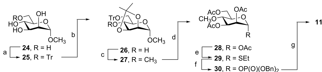
Scheme 3: Reagents and conditions: (a) TrCl, DMAP, pyridine, 85%; (b) DMP, p -TsOH, 76%; (c) \text{CH}_3\text{I} , NaH, DMF, 91%; (d) \text{Ac}_2\text{O} – \text{HOAc} – \text{H}_2\text{SO}_4 , 35:15:1, 55%; (e) EtSH, \text{BF}_3\cdot\text{OEt}_2 , \text{CH}_2\text{Cl}_2 , 70%; (f) \text{HO-P(O)(OBn)}_2 , NIS, AgOTf, \text{CH}_2\text{Cl}_2 , 80%; (g) (i) \text{H}_2 , \text{Pd(OH)}_2\text{-C} , toluene, \text{Et}_3\text{N} , pyridine; (ii) \text{CH}_3\text{OH} – \text{H}_2\text{O} – \text{Et}_3\text{N} , 5:2:1, 70%.
