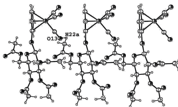
Figure 7: ORTEP-plot of the asymmetric unit showing three molecules of compound 2j and 30% probability ellipsoids; the arrows show the nonclassical H-bonds between O13 and H22a.
