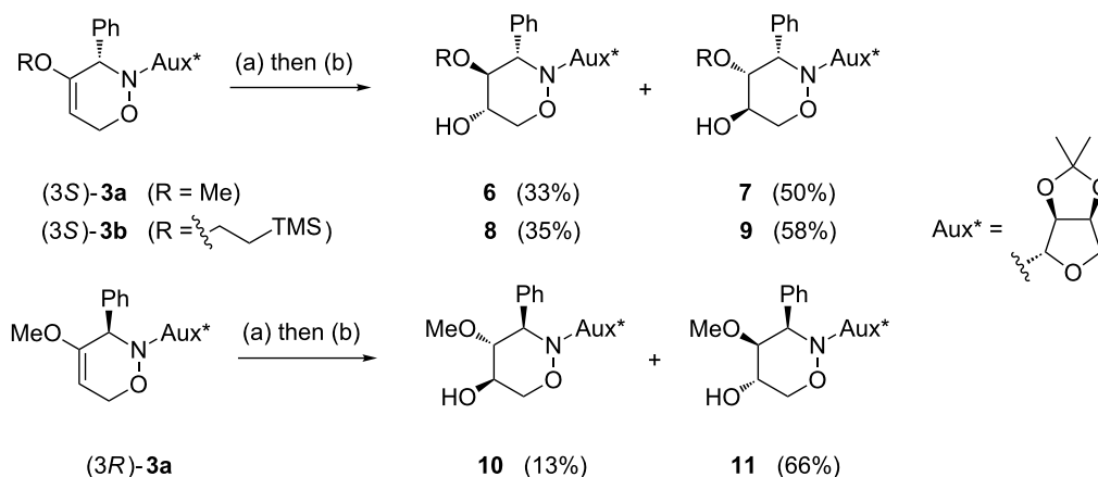
Scheme 4: Introduction of a 5-hydroxy group into 1,2-oxazine derivatives 3 by a hydroboration/oxidation protocol; (a) \text{BH}_3 \cdot \text{THF} (4.0 equiv), THF, -30^\circ\text{C} to rt, 3 h; (b) NaOH, \text{H}_2\text{O}_2 (30%), -10^\circ\text{C} to rt, overnight.
