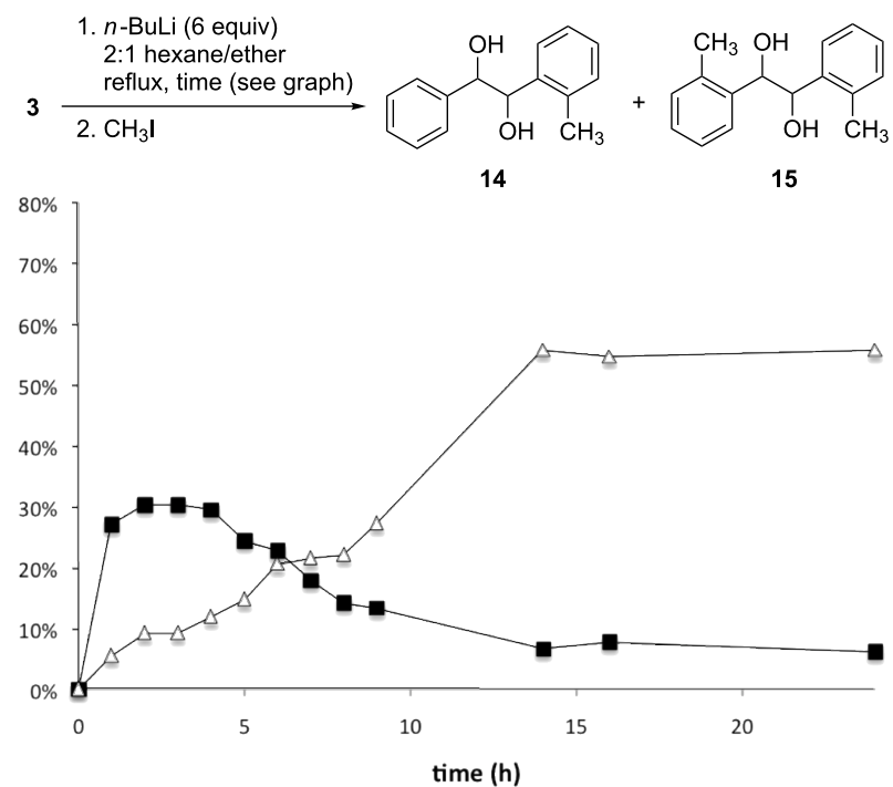
Figure 3: Percentage of methylhydrobenzoin ( 14 ) (■), and dimethylhydrobenzoin ( 15 ) (Δ) as determined by 1 H NMR spectroscopy. The remainder of the material is recovered ( R,R )-hydrobenzoin ( 3 ).
