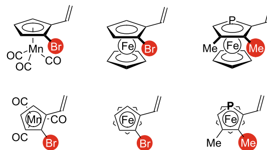
Figure 2: Structures of less-reactive enantiomers in three representative planar-chiral vinylmetallocene substrates in Mo/( R )- L1 -catalyzed AMD/KR.
