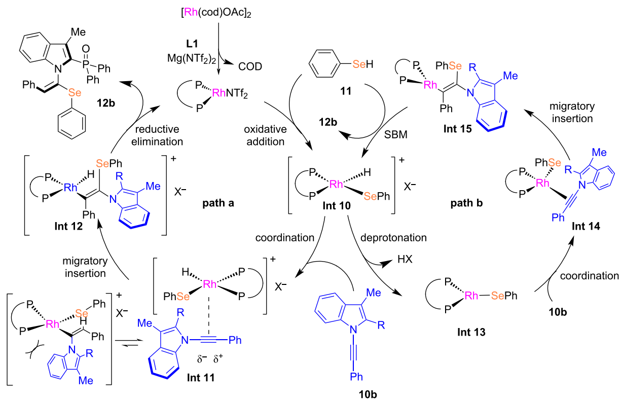
Scheme 4: Rhodium-catalyzed asymmetric hydroseleloration of 1-alkynylindoles. *DCE/DCM 2:1 (v/v), -50 °C.
