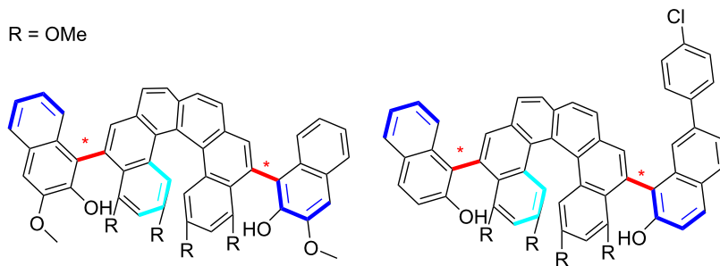
Scheme 15: Synthesis of helicenes containing stereogenic axes.
