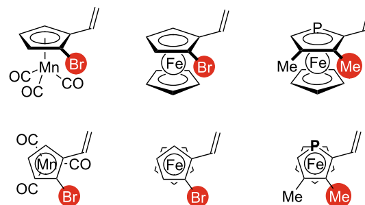
Figure 2: Structures of less-reactive enantiomers in three representative planar-chiral vinylmetallocene substrates in Mo/( R )- L1 -catalyzed AMD/KR.
