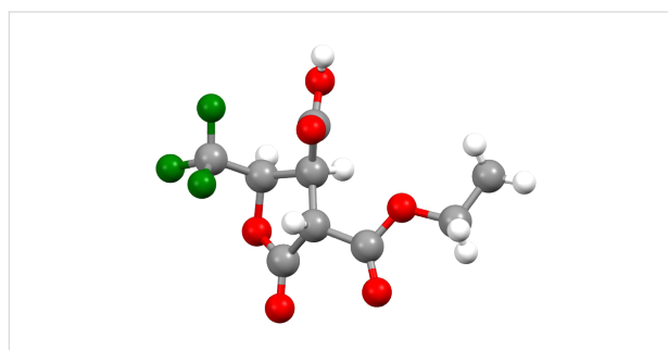
Figure 2: Crystallographic structure of anti,syn-8a .
