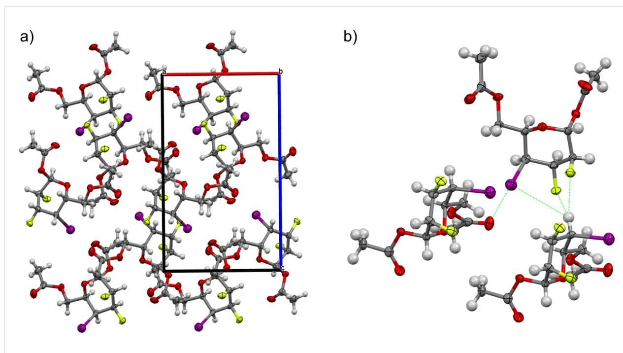
Figure 4: Packing arrangement of compound compound 15 ; a) View down the b axis; b) proposed intermolecular interactions involving halogens. ORTEP diagram showing 50% thermal ellipsoid probability: carbon (gray), oxygen (red), fluorine (green), iodine (purple), and hydrogen (white).
