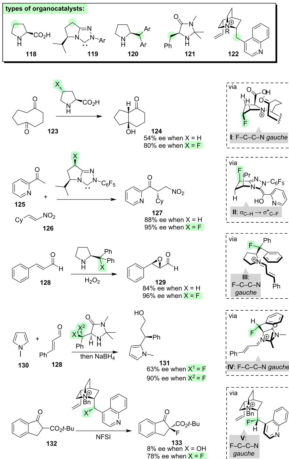
Figure 13: Effects of incorporating fluorine into organocatalysts.
