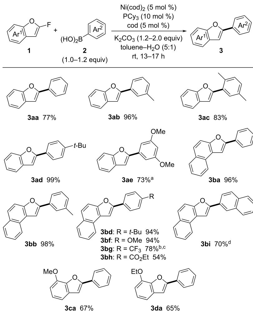
Scheme 2: Synthesis of 2-arylbenzofurans 3 via the coupling of 1 with 2 . Isolated yields are given. a \text{Ni}(\text{cod})_2 (10 mol %), \text{PCy}_3 (20 mol %), and \text{cod} (10 mol %). b \text{Ni}(\text{cod})_2 (20 mol %), \text{PCy}_3 (40 mol %), and \text{cod} (20 mol %). c \text{K}_3\text{PO}_4 (1.2 equiv) was used as a base. d Toluene–MeOH– \text{H}_2\text{O} (5:1:1) was used as a solvent.
