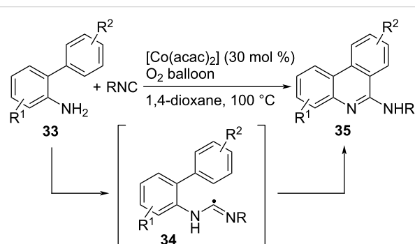
Scheme 27: Phenanthridine synthesis by oxidative cyclization of 2-aminobiphenyls.
