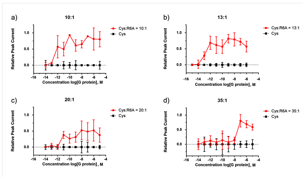
Figure 11: Calibrating the array-based signaling experiment for monitoring small molecule G-protein interactions.
