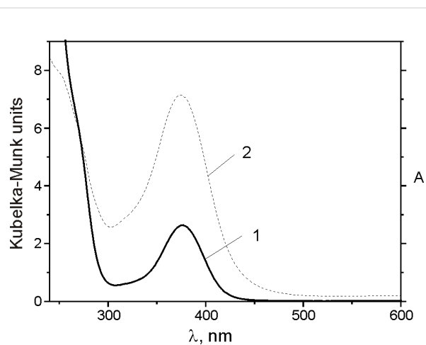
Figure 6: UV–vis spectra of 3 /SBA-15 (curve 2) and of 3 (curve 1) in dichloromethane ( c = 0.001\text{ mol/L} , l = 0.2\text{ cm} ).
