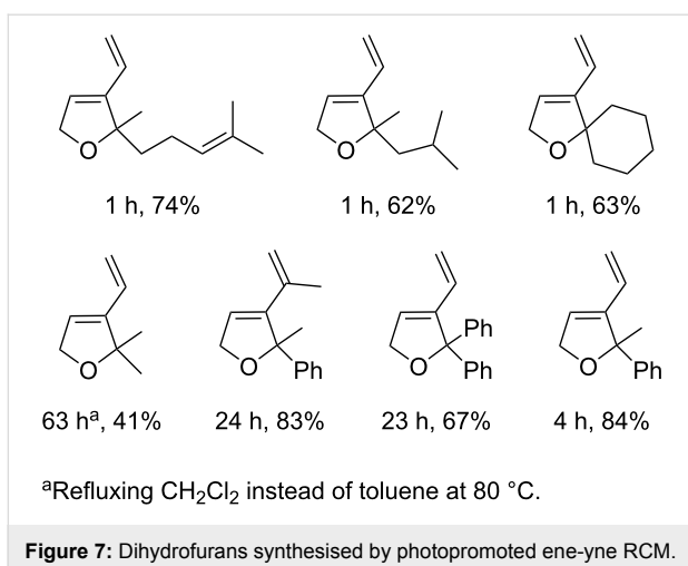
Scheme 4: Photopromoted ene-yne RCM by cationic allenylidene ruthenium complex 14 .
