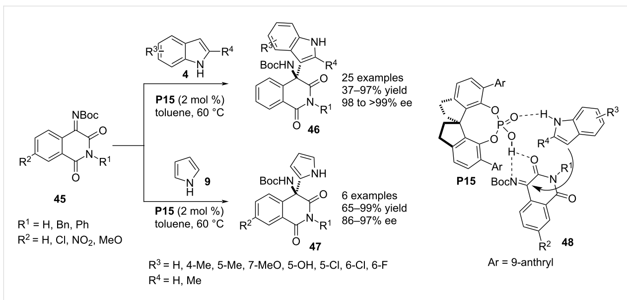
Scheme 13: Isoquinoline-1,3(2 H ,4 H )-dione scaffolds as electrophiles.
