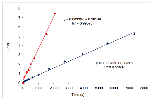
Figure 2: Second-order kinetics plot for the addition of TMSCN to benzaldehyde at 0 °C catalysed by complex 2 in dichloromethane (red) and propylene carbonate (blue). The units for the vertical scale are \ln[(B_0A_t)/(B_tA_0)]/(A_0 - B_0) , where A = [PhCHO], B = [Me 3 SiCN], and the subscripts 0 and t refer to initial concentrations and concentrations at time t, respectively.
