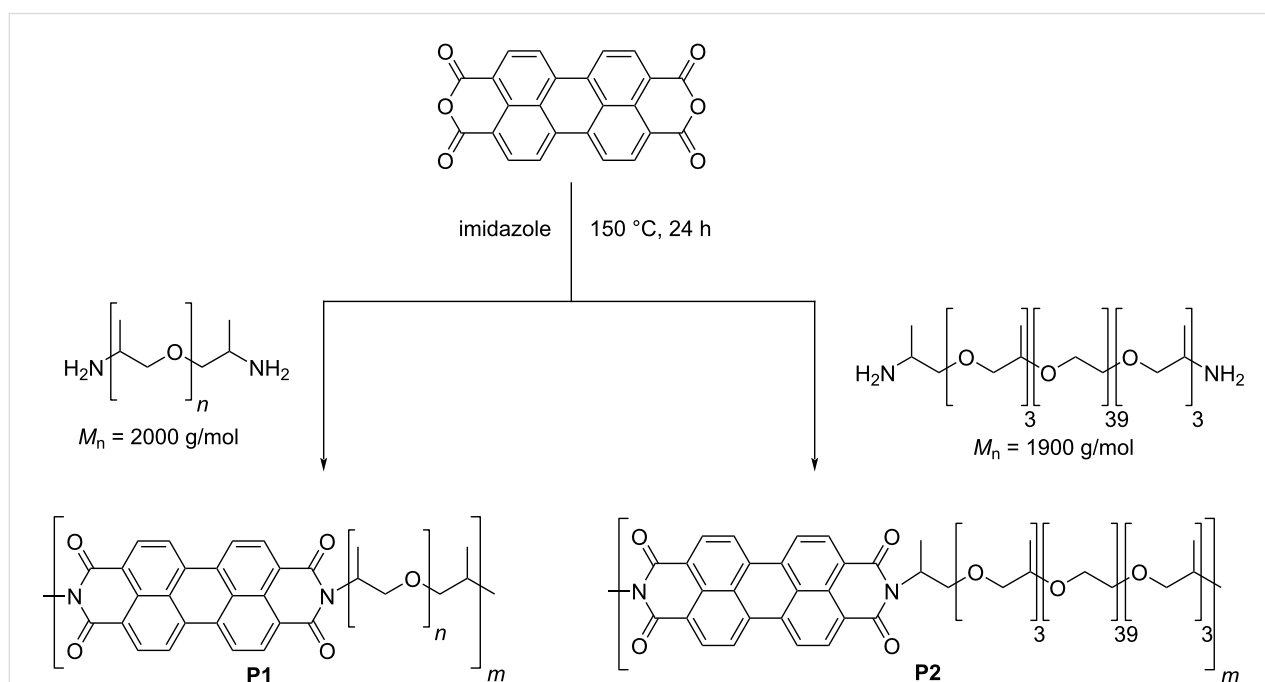
Scheme 1: Schematic representation of the polymer synthesis of P1 and P2 .
