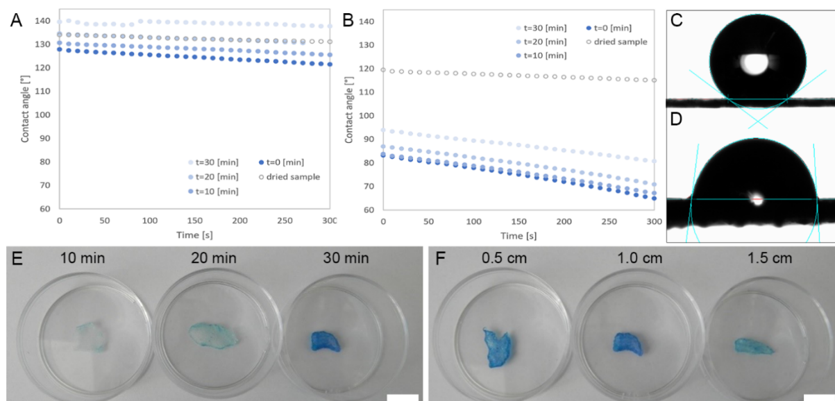
Figure 1: A) Graph showing change in the static contact angle with time on a pristine PCL scaffold with a 500 µm hatch spacing and B) on a SIPGP-coated scaffold with a 500 µm hatch spacing. The measured samples were immersed in water for different periods of time t = 0, 10, 20, 30 [min]. C) Photograph of a 2 µL water drop on a pristine PCL scaffold immediately after droplet deposition and D) on a SIPGP-modified scaffold immediately after droplet deposition. E and F) toluidine blue staining of PCL scaffolds coated with PHEMA via SIPGP showing the variation with E) the UV-reaction time and F) the distance between light source and substrate. Scale bar for E and F is 1 cm.
