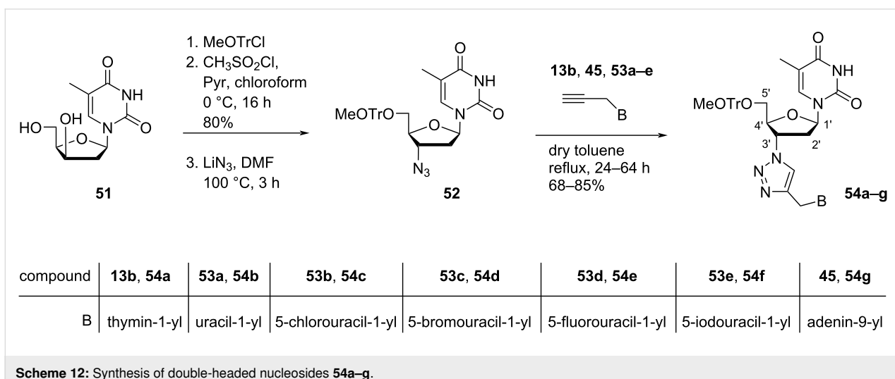
Scheme 12: Synthesis of double-headed nucleosides 54a–g .
