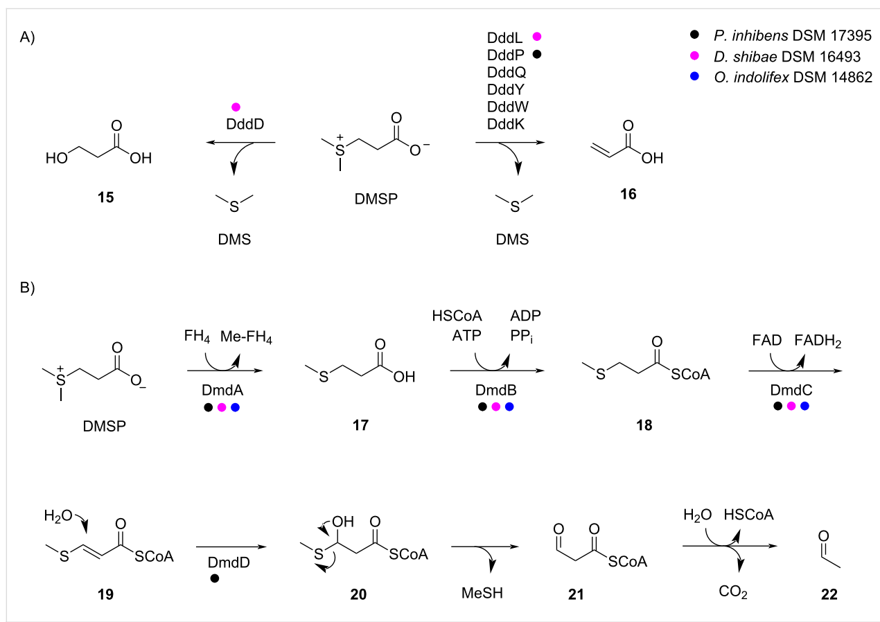
Scheme 2: Degradation of DMSP by marine bacteria. A) Hydrolysis or lysis to DMS, B) demethylation pathway leading to MeSH. The color code shows which enzymes are encoded in the genomes of the strains investigated in this study.
