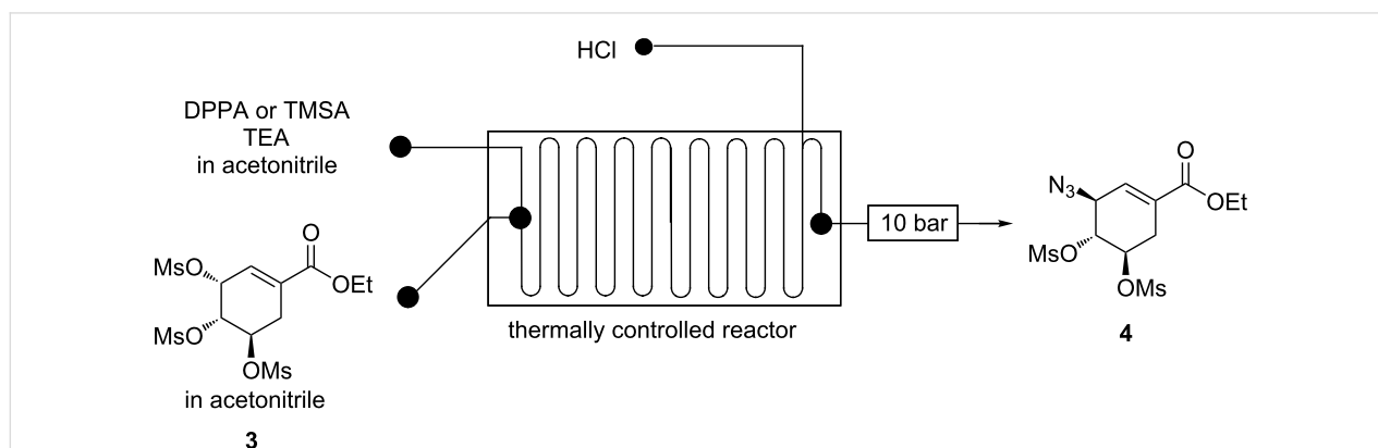
Figure 7: Continuous-flow system for C-3 azidation of mesyl shikimate using DPPA or TMSA.
