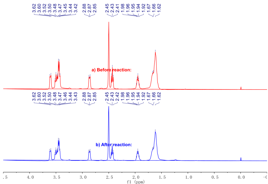
Figure 3: ^1\text{H} NMR (400 MHz, \text{DMSO-}d_6 ) spectra of [\text{HSO}_3\text{-BDBU}]\text{H}_2\text{PO}_4 : a) Fresh one; b) used one after five cycles.
